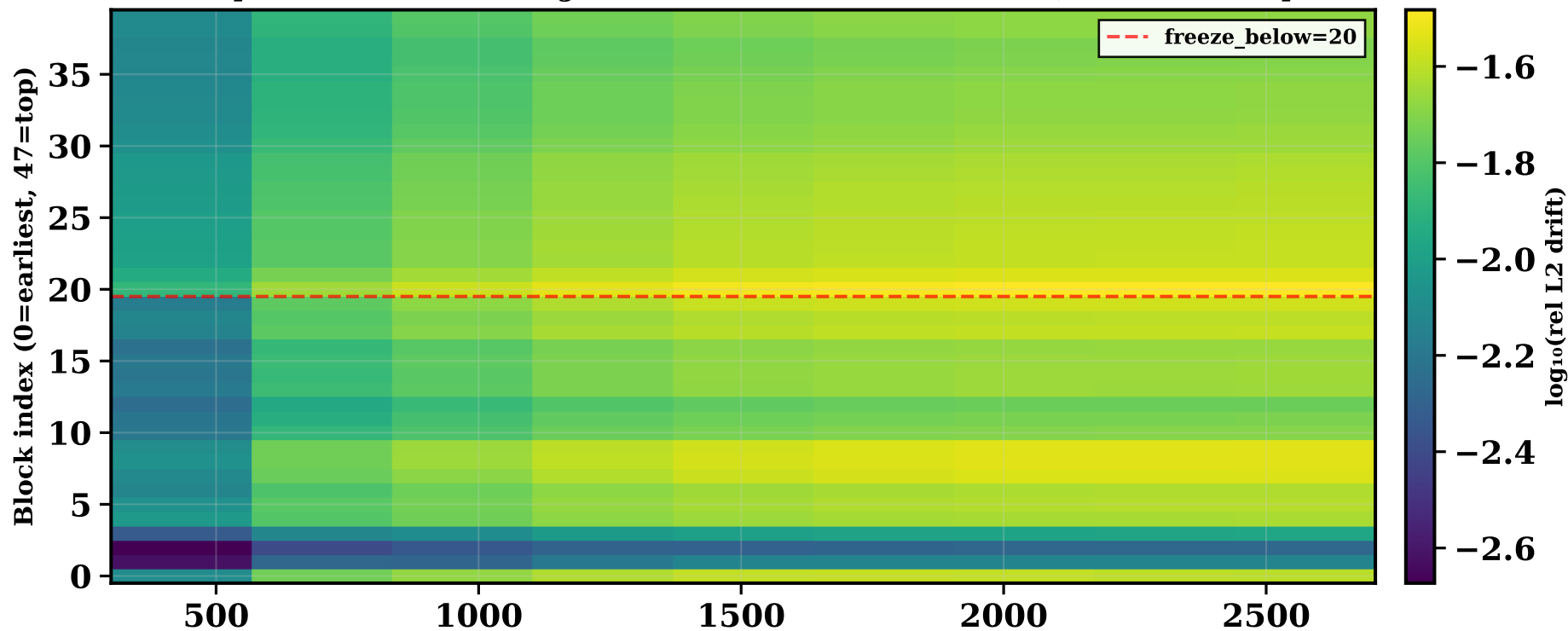
m09a step=2708 · Per-block weight drift vs Meta init (rows=blocks, cols=val checkpoints)
