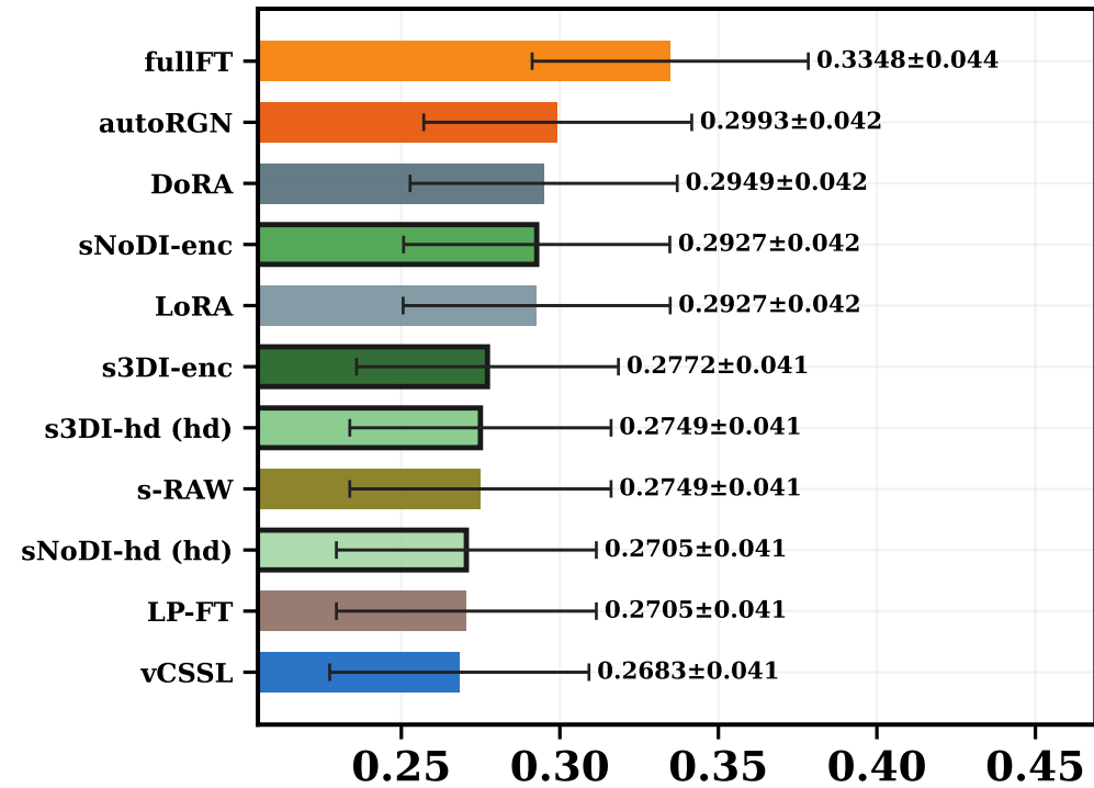
action top-1 ↑ · best: fullFT
