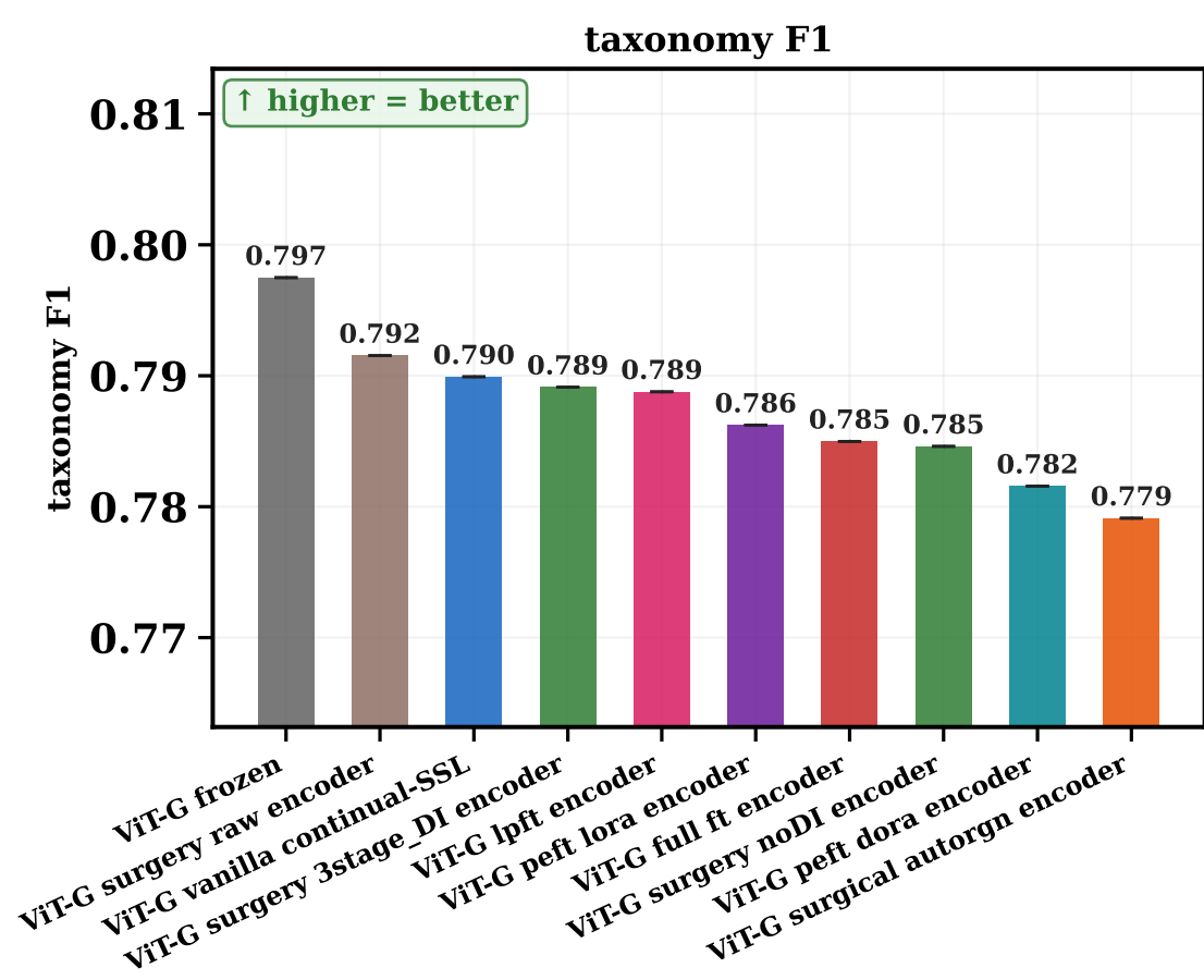
iter18 EVAL scorecard — per-encoder TEST artifacts · 95% BCa CI where available
