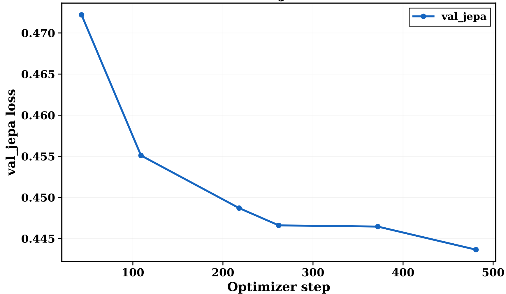
m09c · \lambda=0.005 · Validation JEPa loss + kill-switch state
