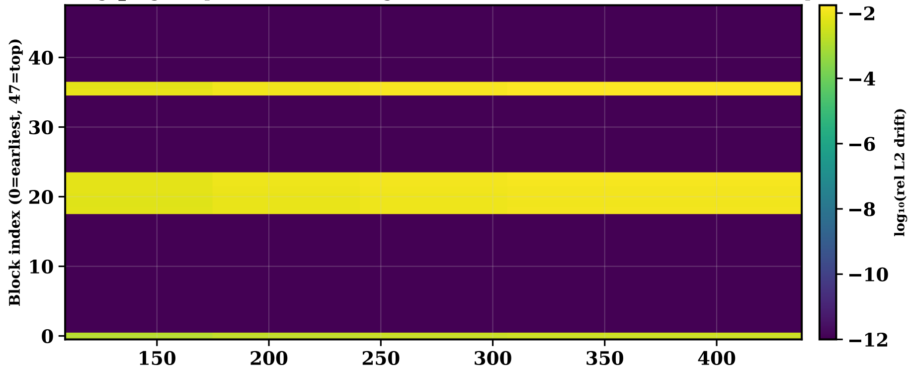
m09c autorgn_single step=438 · Per-block weight drift vs Meta init (rows=blocks, cols=val checkpoints)
