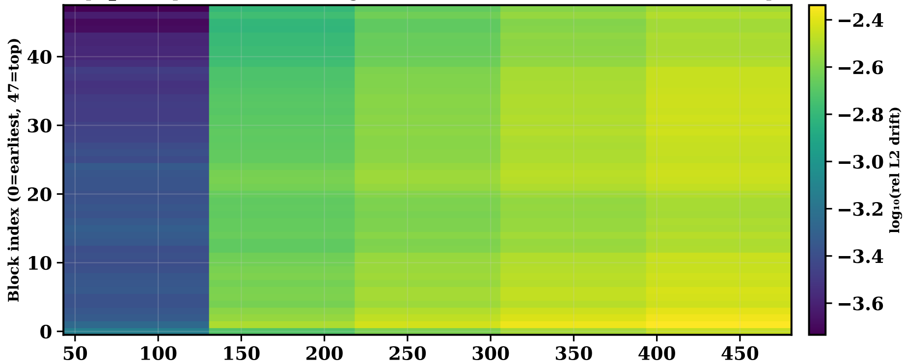
m09c lpft_full step=481 · Per-block weight drift vs Meta init (rows=blocks, cols=val checkpoints)
