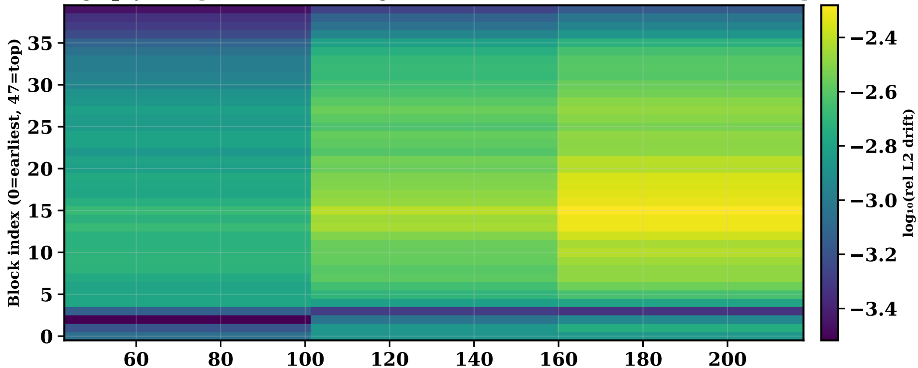
m09c stage1_layout step=218 · Per-block weight drift vs Meta init (rows=blocks, cols=val checkpoints)
