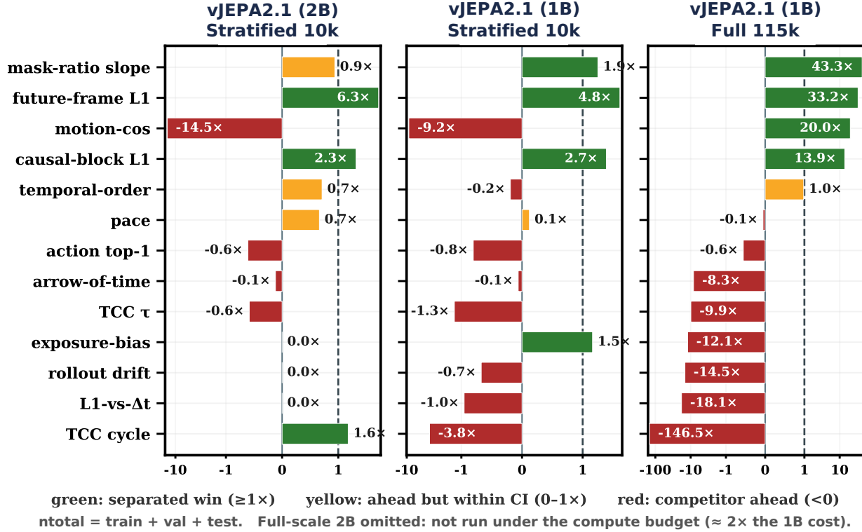
Figure 5: FactorJEPA vs. the best competitor, across scale. Per-metric advantage in 95%-CI units at the stratified 10k scale (2B and 1B) and the full 115k scale (1B); green past the dashed 1× line = a separated win. Predictive diagnostics separate and strengthen at full scale, where the motion-cosine trade-off also reverses to a win. Full-scale 2B was not run (compute budget).
