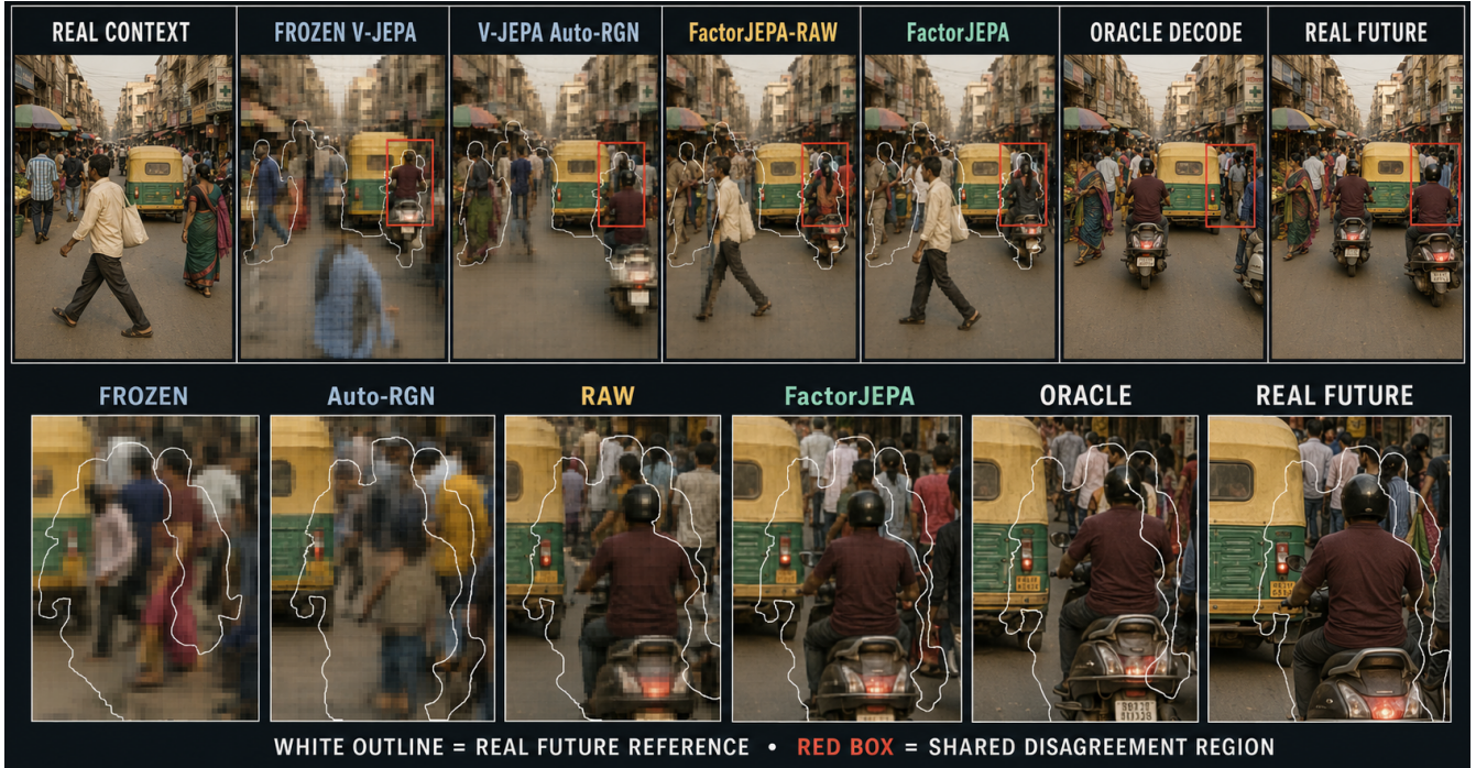
Figure 12: Illustrative layout for future-consistency inspection. The top row compares the observed context with decoded futures from frozen V-JEPA, V-JEPA Auto-RGN, FactorJEPA-RAW, and FactorJEPA, followed by the target-latent oracle reconstruction and observed future. The identical white contour, derived from the observed future, is overlaid on every predicted panel to expose disagreement in agent occupancy, position, visibility, and interaction geometry. Red boxes identify a common high-disagreement region, enlarged in the bottom row. The synthesized panels demonstrate the intended visualization protocol and are not experimental model outputs.
