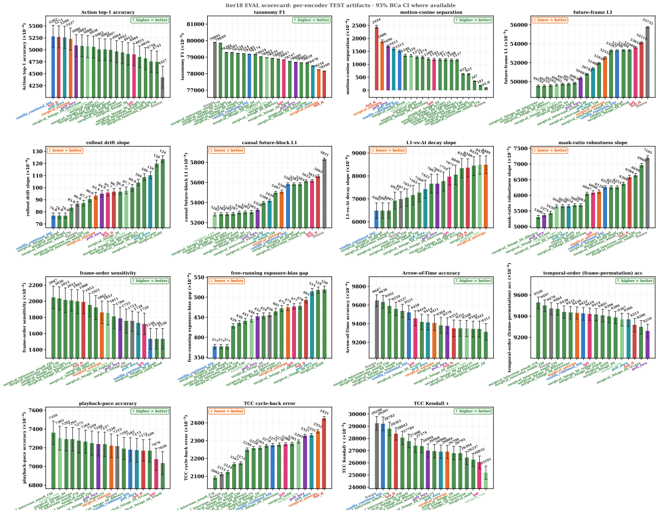
Figure 11: Complete ViT-G attribution and ablation scorecard. The comparison includes frozen and continually adapted V-JEPA, full and parameter-efficient fine-tuning, Auto-RGN, FactorJEPA-RAW, the executed FactorJEPA objective variants, and the WiseFT encoder-scope variants. Bars report held-out means; error bars denote 95% BCa confidence intervals where available. Each panel states whether higher or lower values are preferred. Internal variants are mapped to their publication-facing definitions in Table 6. Attribution claims use the prespecified contrasts in Table ??, rather than selecting the best method separately for each diagnostic.
