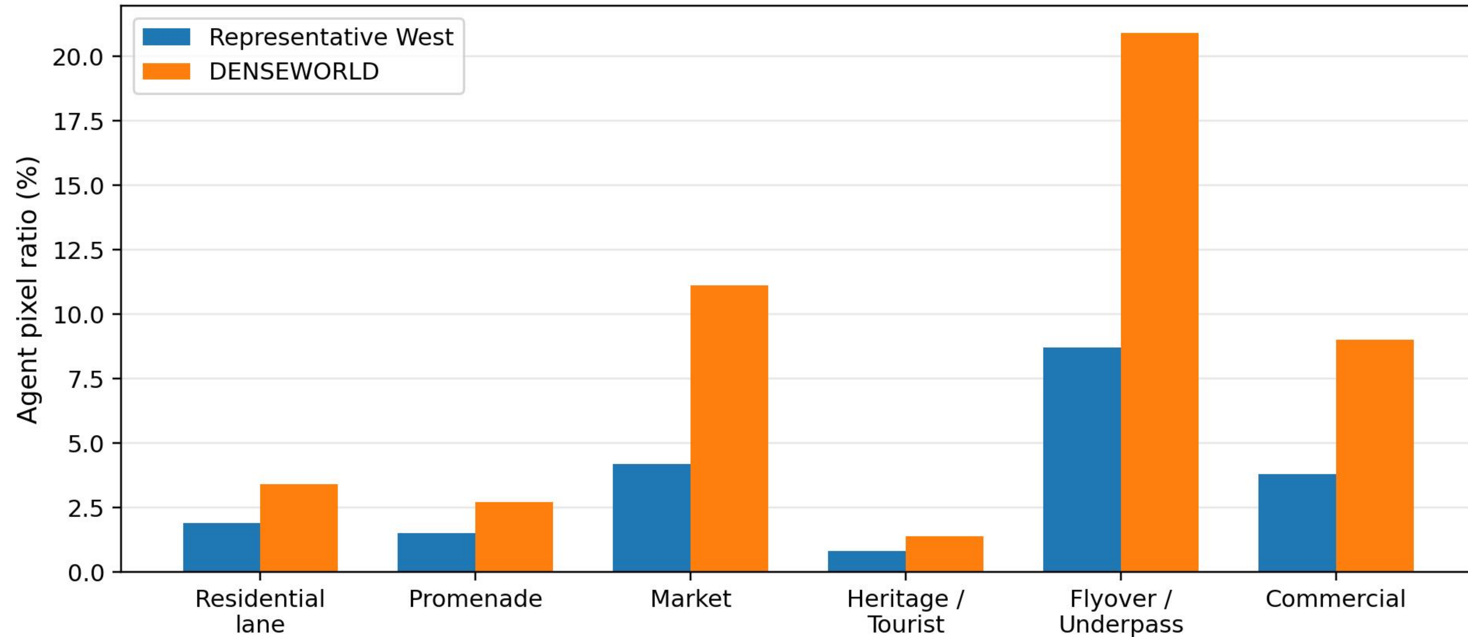
Agent Occupancy
