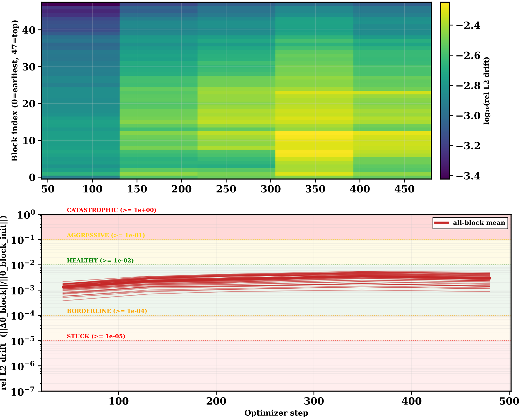
m09c stage3_interaction step=480 · Per-block weight drift vs Meta init (rows=blocks, cols=val checkpoints)
