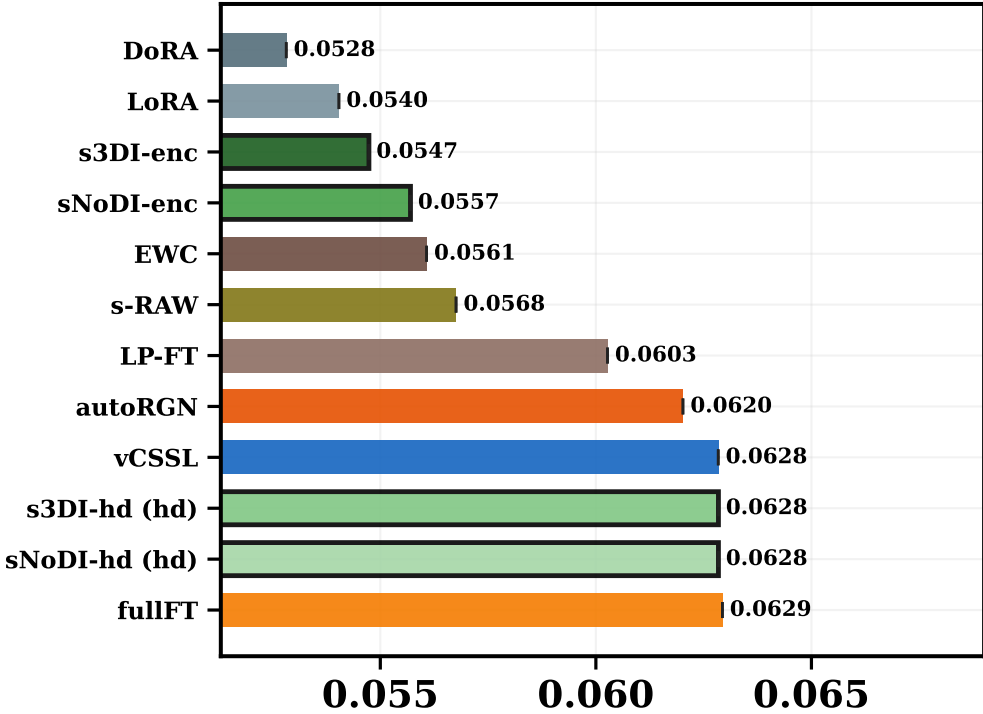
mask-ratio ↓ · best: DoRA
