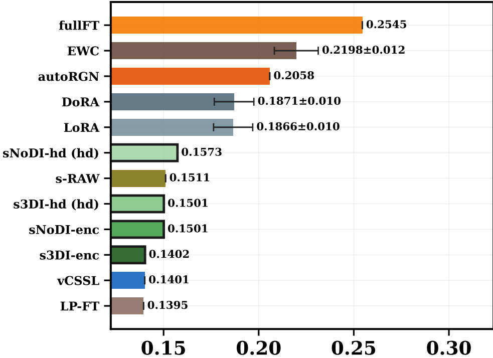
motion-cos ↑ · best: fullFT
