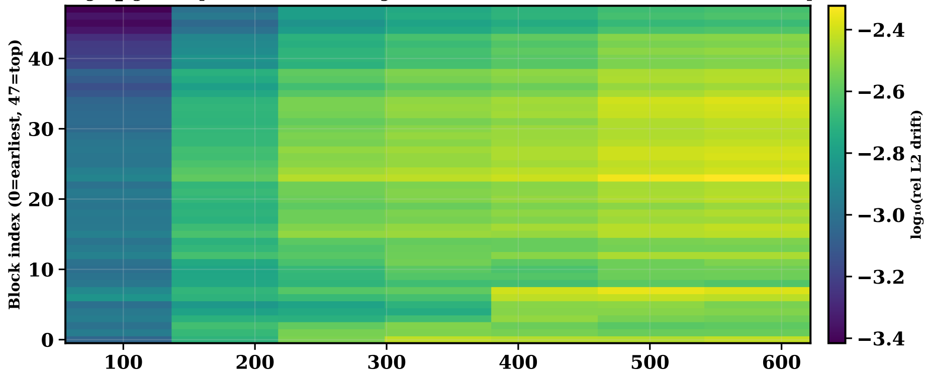
m09c stage2_agent step=622 · Per-block weight drift vs Meta init (rows=blocks, cols=val checkpoints)
