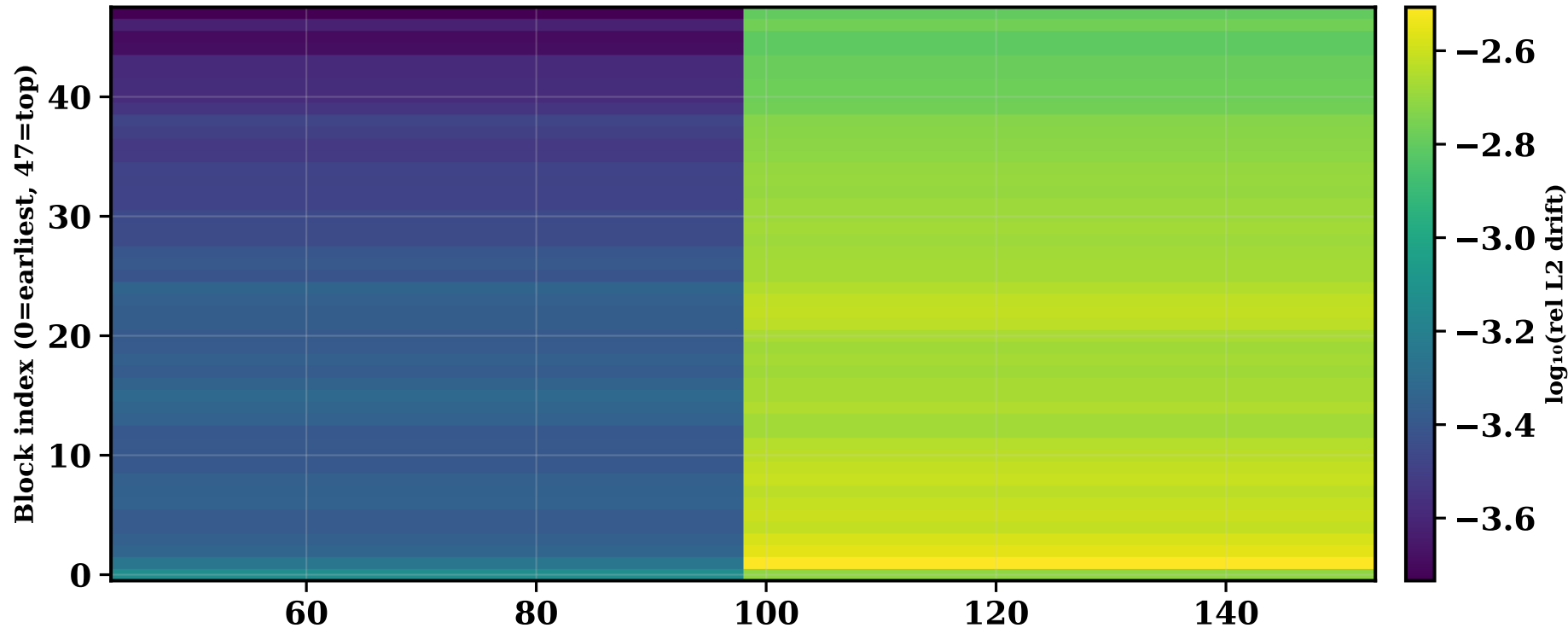
m09c lpft_full step=153 · Per-block weight drift vs Meta init (rows=blocks, cols=val checkpoints)
