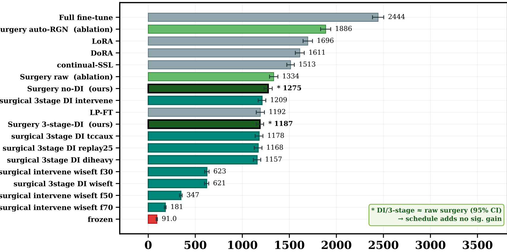
Motion-cosine (motion coherence) (↑ higher better) (×10 -4 )
