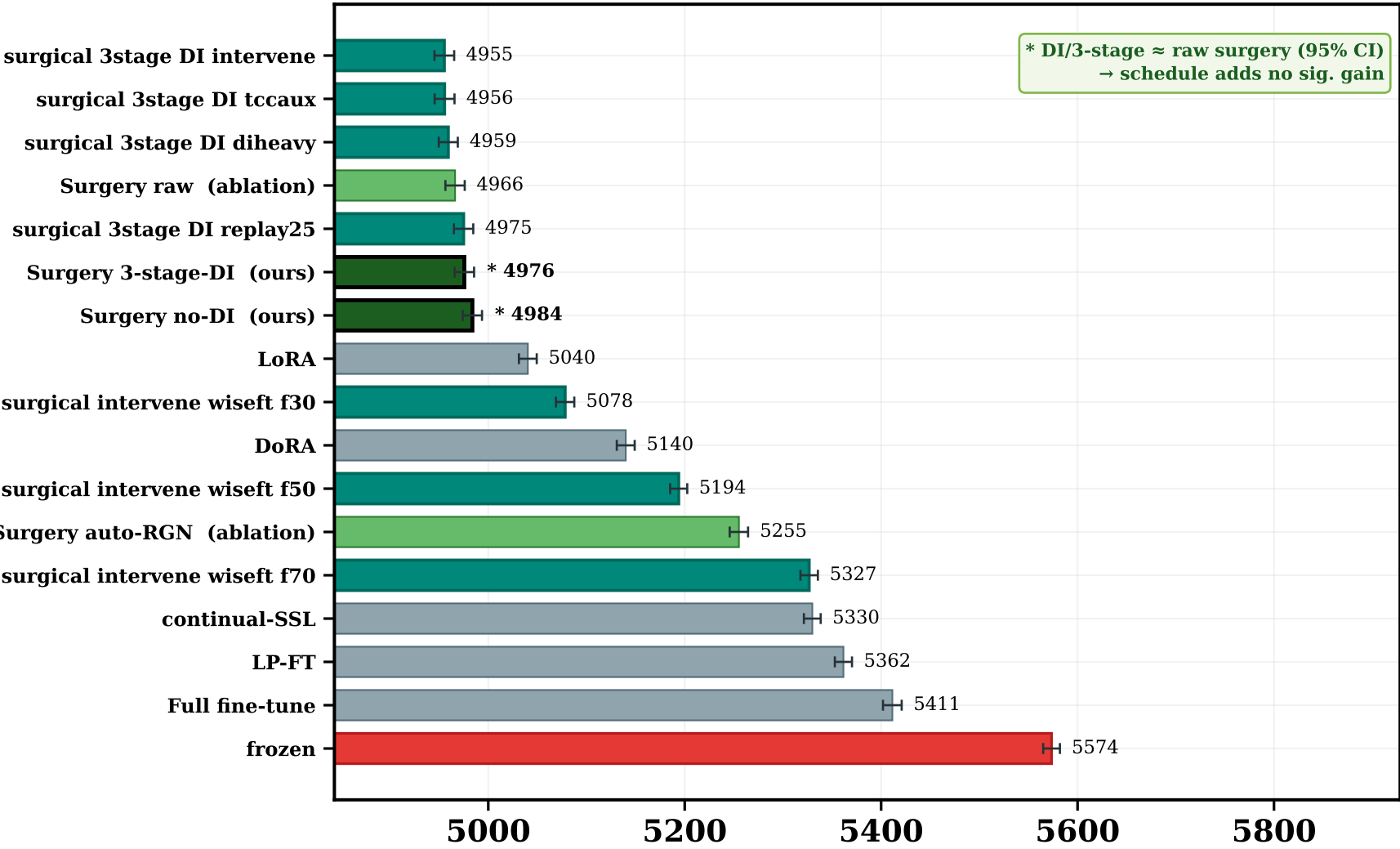
HERO · Future-frame MSE (world-model prediction) (↓ lower better) (×10 -4 )
