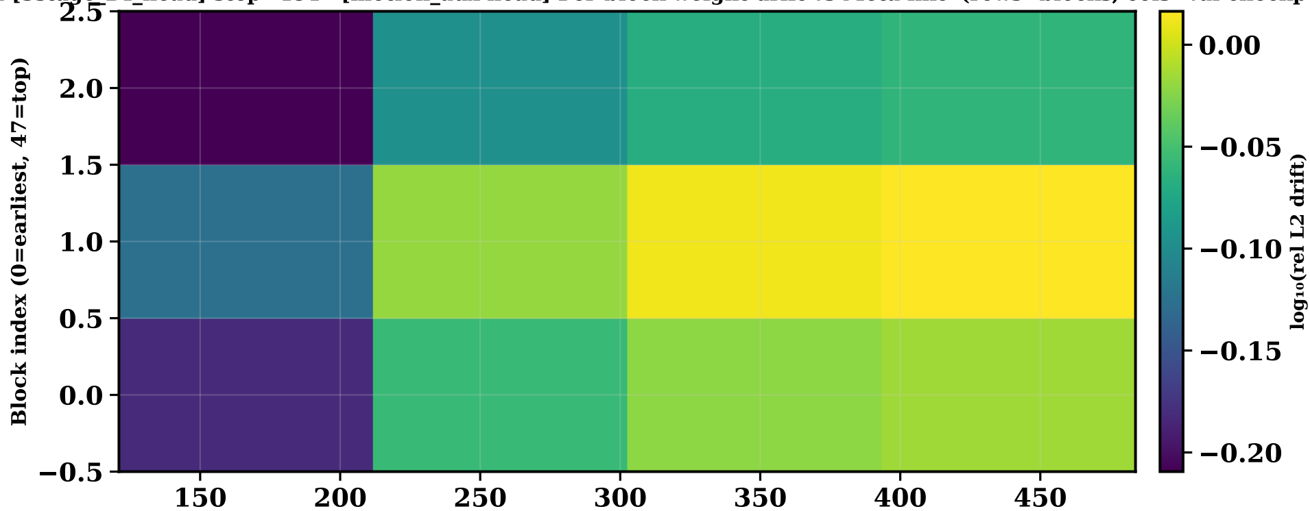
m09c head [3stage_DI_head] step=484 · [motion_aux head] Per-block weight drift vs Meta init (rows=blocks, cols=val checkpoints)
