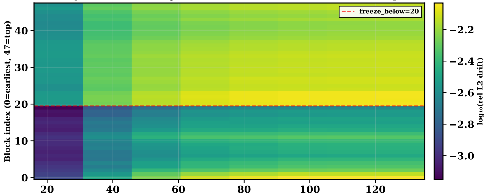
m09a step=135 · Per-block weight drift vs Meta init (rows=blocks, cols=val checkpoints)
