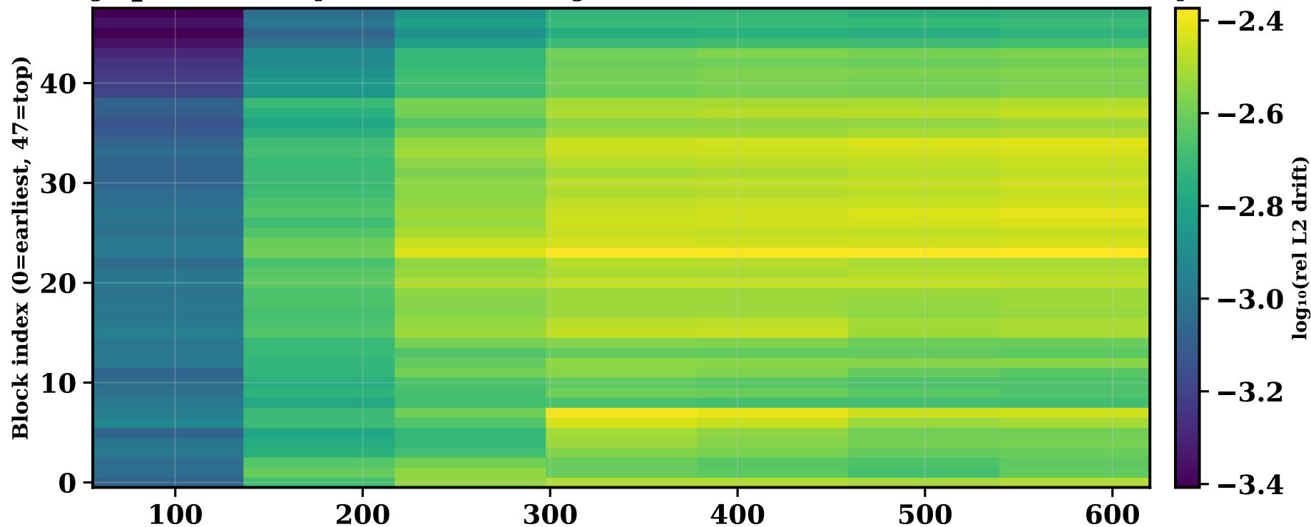
m09c stage3_interaction step=620 · Per-block weight drift vs Meta init (rows=blocks, cols=val checkpoints)
