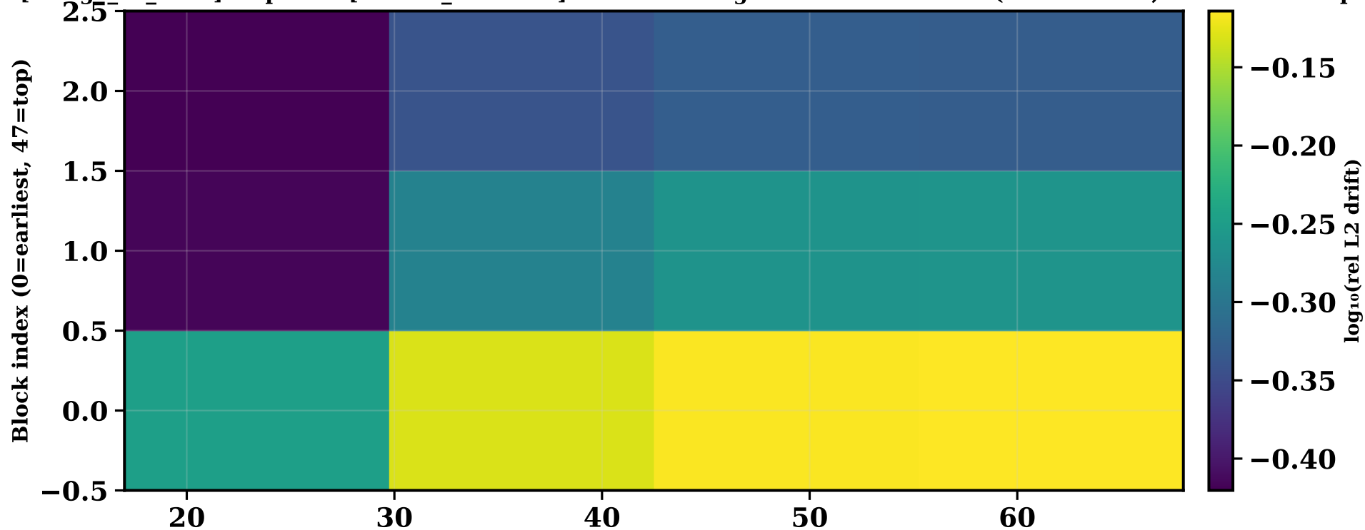
m09c head [3stage_DI_head] step=68 · [motion_aux head] Per-block weight drift vs Meta init (rows=blocks, cols=val checkpoints)
