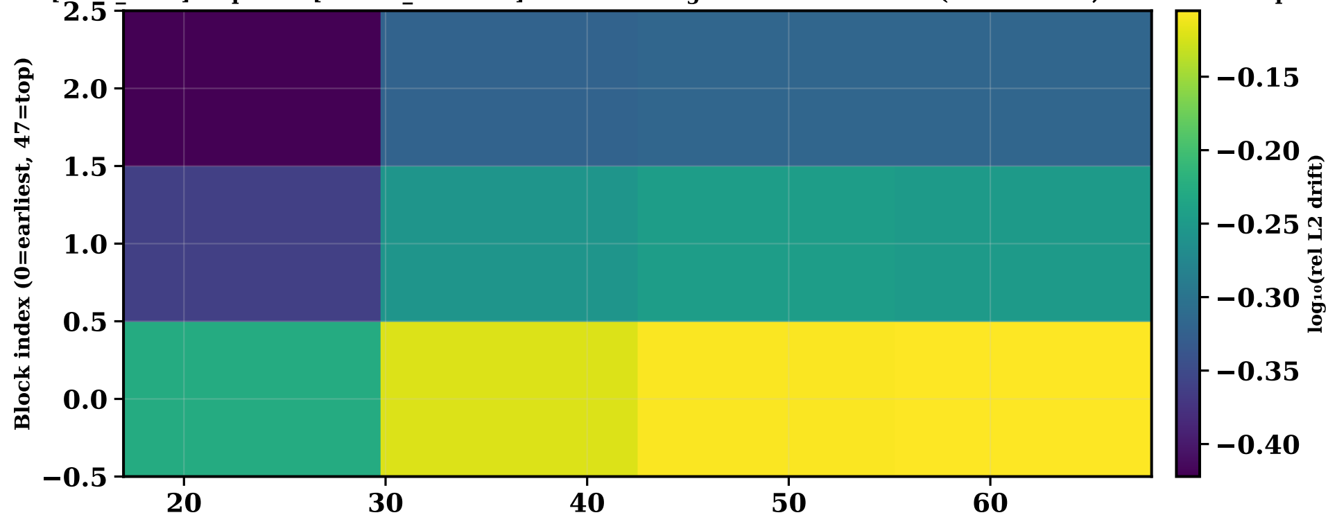
m09c head [noDI_head] step=68 · [motion_aux head] Per-block weight drift vs Meta init (rows=blocks, cols=val checkpoints)
