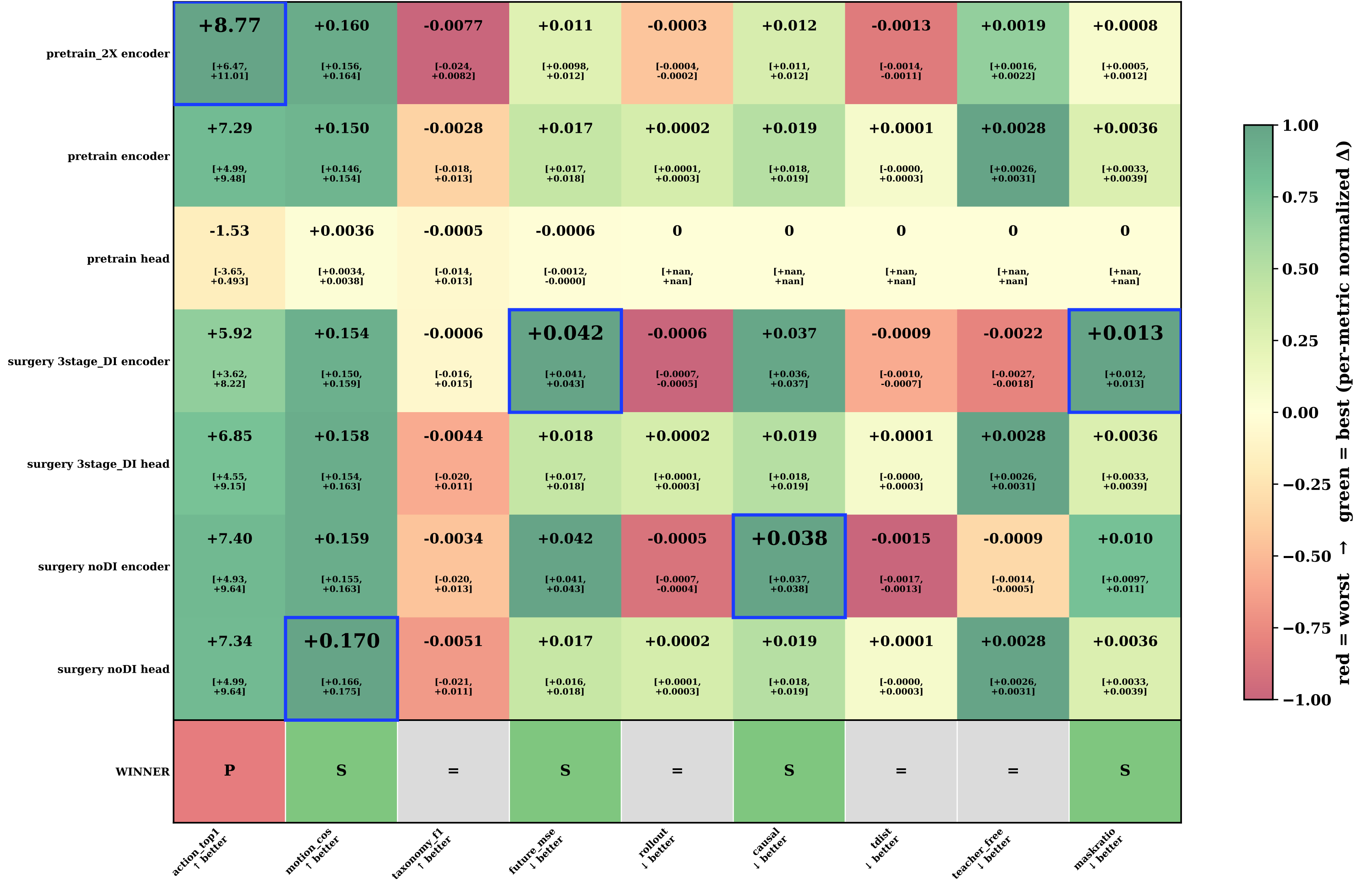
HERO — \Delta vs V-JEPA 2.1 frozen · per cell: \Delta (top) and 95% BCa CI (bottom), sign-corrected so + = better colour: red = worst, green = best (per-metric min-max) · column badge \uparrow/\downarrow = better-direction · BLUE BOX + big \Delta = champion-duel winning arm (none on ties — matches WINNER row)
