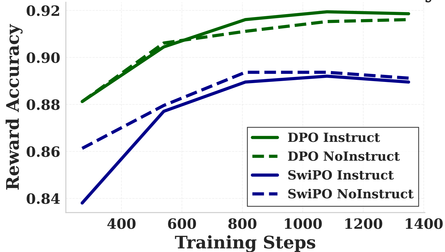
DPO / SwiPO: Reward Accuracy
