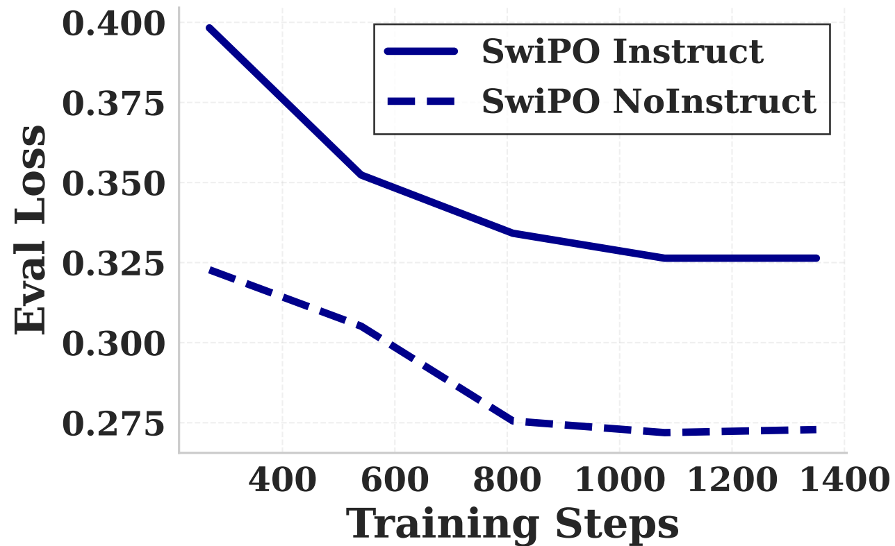
SwiPO
