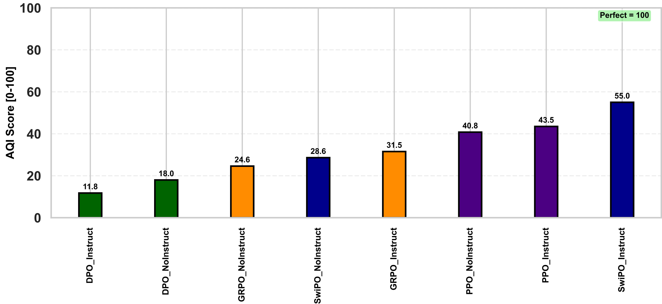
AQI: Alignment Quality Index (Higher = Better) (Llama-3.1-8B)
