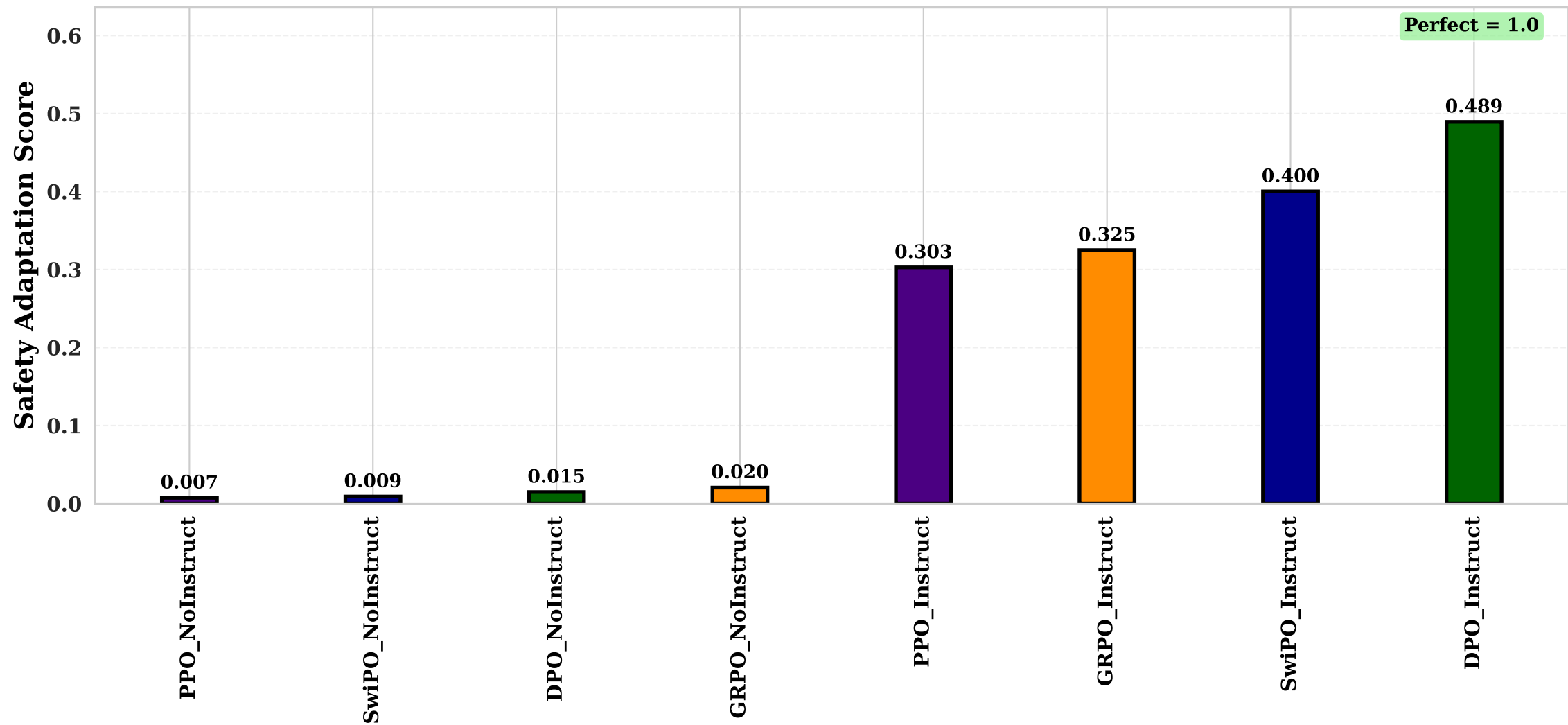
Conditional Safety: Adaptation Score (Higher = Better) (Llama-3.1-8B)
