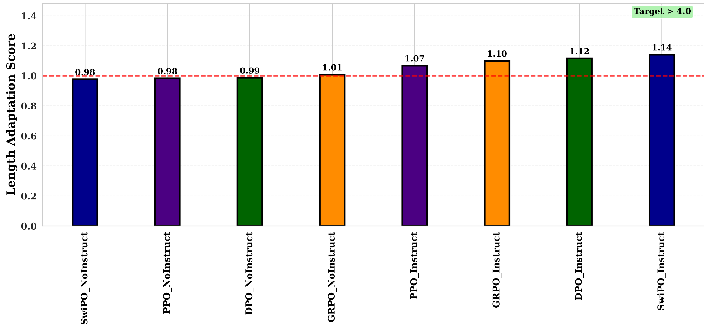
Length Control: Adaptation Score (Higher = Better) (Llama-3.1-8B)
