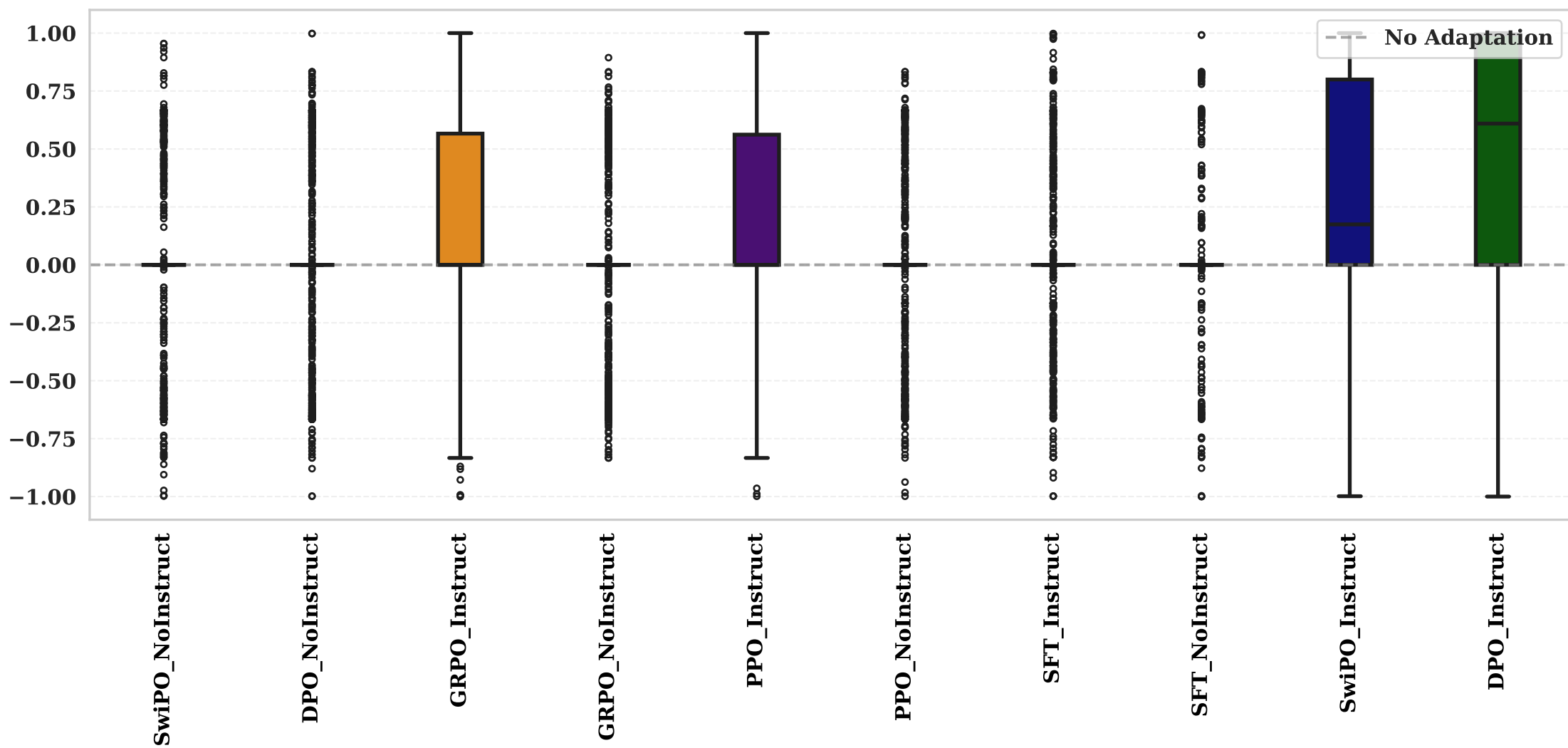
Conditional Safety: Adaptation Score Distribution (Llama-3.1-8B) (Box Plot)
