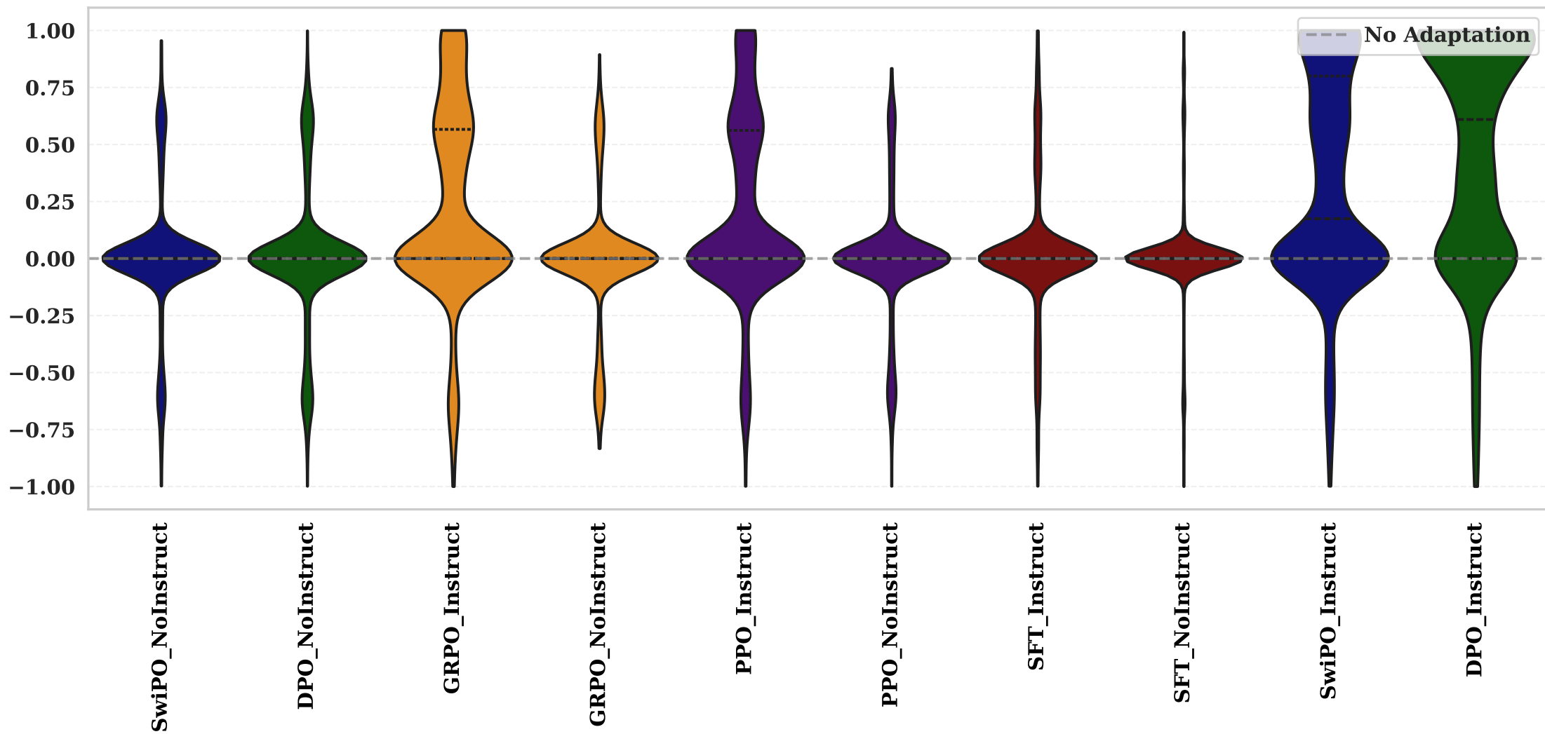
Conditional Safety: Adaptation Score Distribution (Llama-3.1-8B) (Violin Plot)
