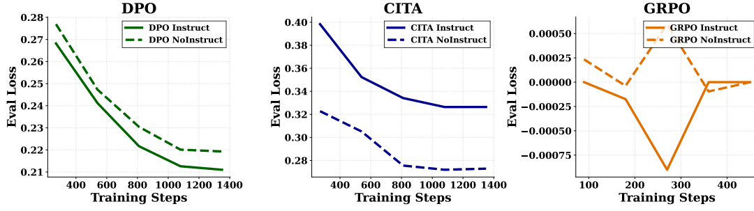
Figure 20: Evaluation loss across policy optimization methods. We plot evaluation loss for DPO, CITA, and GRPO using independent y-axes due to non-comparable loss scales. DPO (left): loss \sim 0.21 – 0.28 with smooth convergence; the Instruct variant is slightly lower, consistent with stronger preference fit under the instruction-augmented setup. CITA (center): loss \sim 0.27 – 0.40 ; the NoInstruct curve converges lower, while CITA_INSTRUCT attains larger reward margins, reflecting a separation–stability trade-off induced by the mandatory anchoring term. GRPO (right): loss oscillates near zero ( \pm 0.001 ), characteristic of online RL training where the objective is dominated by on-policy sampling variance. Note: PPO tensorboard logs were empty due to a TRL logging issue, so we do not include PPO curves here.
