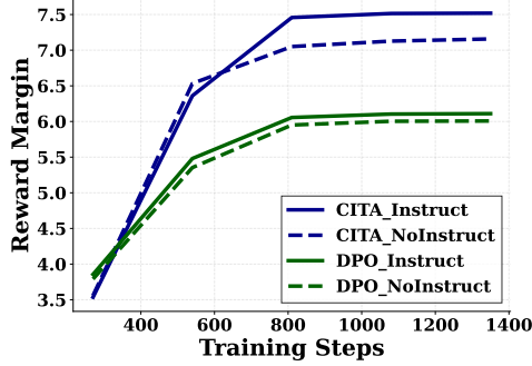
Figure 5: Preference reward margins. \text{CITA}_{\text{Instruct}} (\sim 7.5) > \text{CITA}_{\text{NoInstruct}} (\sim 7.2) > \text{DPO} (\sim 6.0) . Higher margins indicate sharper preference separation; the KL anchor is designed to prevent this separation from degenerating into a single dominant regime.
