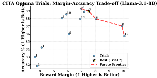
Figure 16: Pareto frontier across trials. Trial 7 lies on the frontier, achieving near-optimal balance (margin=7.52, accuracy=89%) while maintaining strong instruction-conditioned switching.
