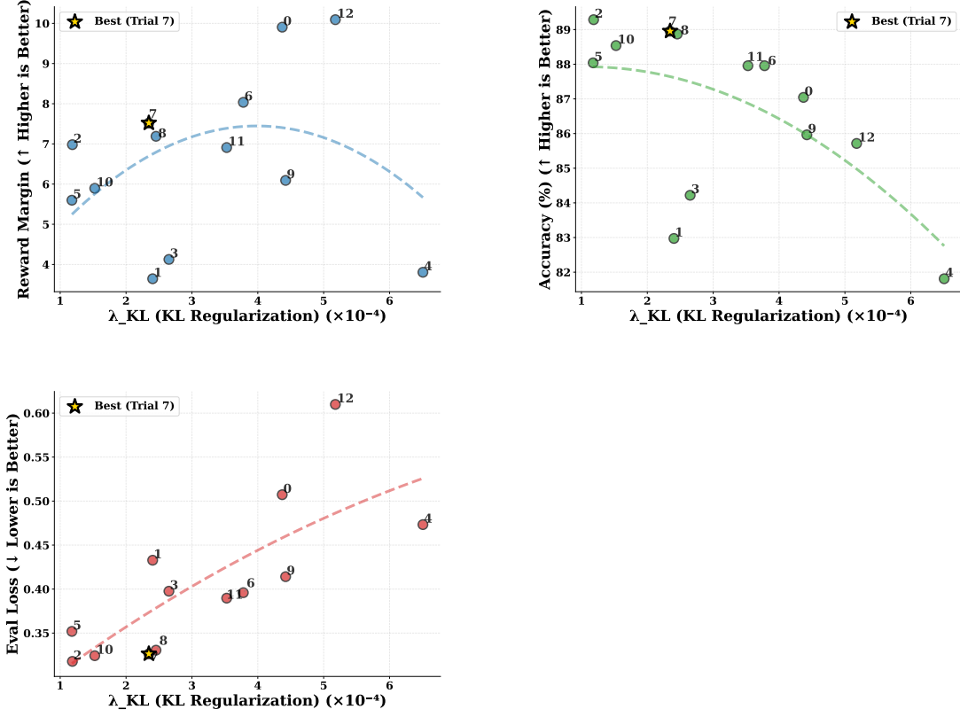
Figure 18: \lambda_{\text{KL}} sensitivity. Reward margin exhibits an inverted-U: too low produces instability and regime interference; too high suppresses learning. Accuracy is comparatively stable, indicating the dominant effect is on switching stability rather than raw preference fit. Trial 7 (★) at \lambda_{\text{KL}}=0.00023 lies in the optimal band.
