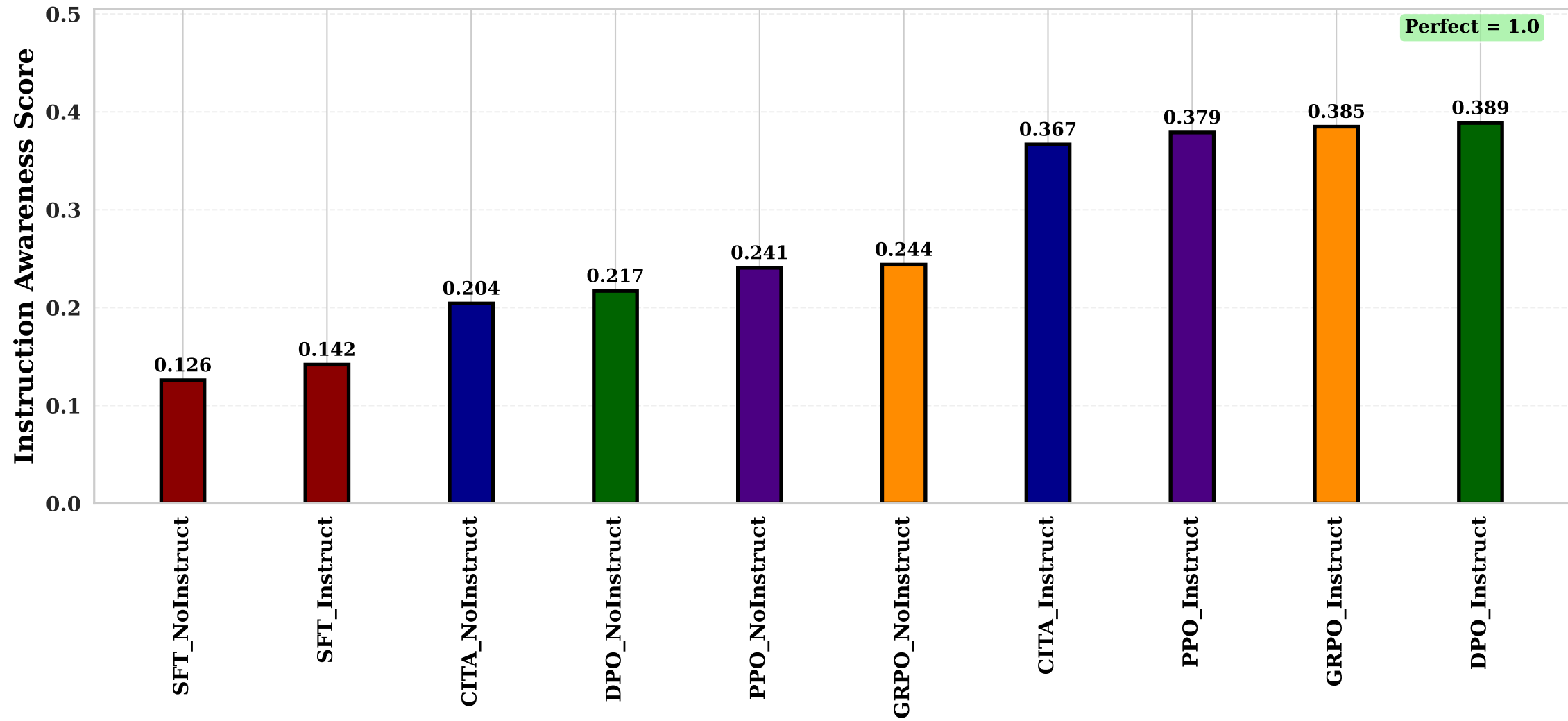
ISD: Instruction Awareness (Higher = Better)
