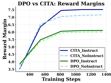
Figure 4: Reward margins. CITA_I (7.5) > CITA_NI (7.2) > DPO (~6.0).
