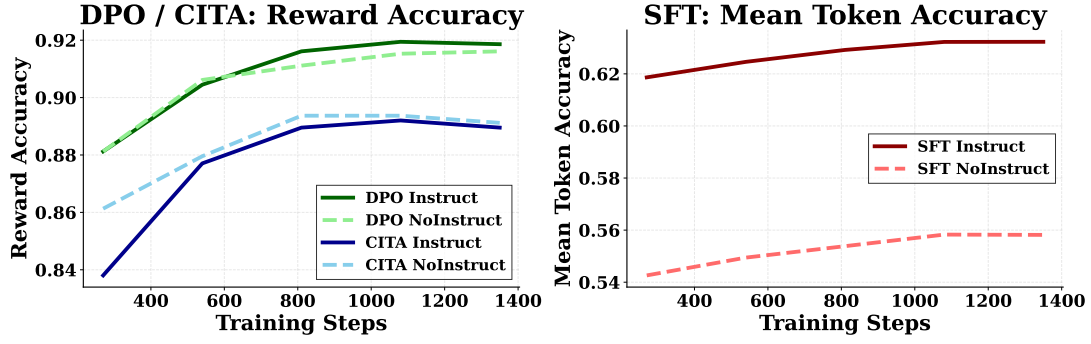
Figure 14: Training Accuracy Metrics: 1 \times 2 subplot comparing accuracy across methods. Left (DPO/CITA): Reward accuracy—all models converge to 89–92%, with DPO variants achieving slightly higher accuracy. Right (SFT): Mean token accuracy—both variants converge smoothly, with Instruct achieving marginally higher accuracy due to richer training signal from instruction-augmented sequences.
