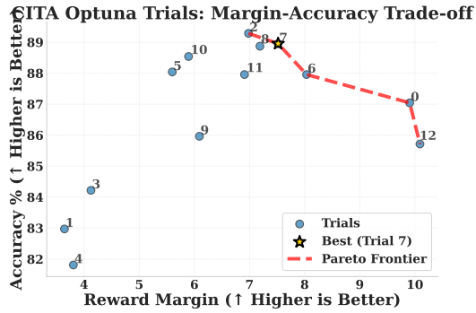
Figure 17: Pareto Frontier: Margin vs. accuracy trade-off across trials. Trial 7 lies on the Pareto frontier, achieving near-optimal balance (margin=7.52, accuracy=89%).
