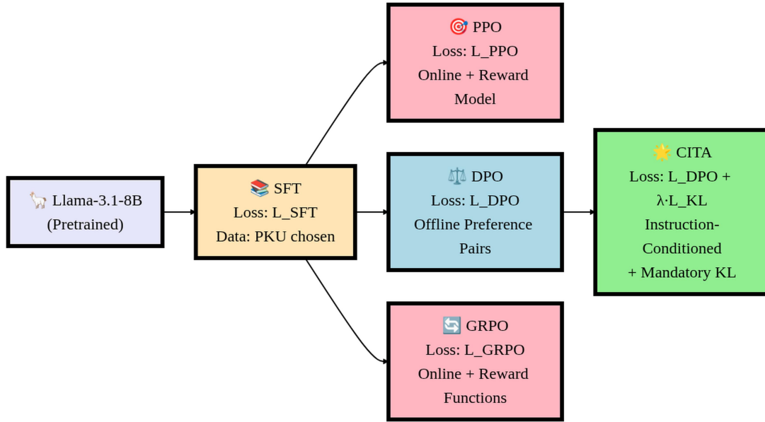
Figure 12: Training Pipeline: All methods branch from SFT. PPO and GRPO are online methods requiring reward model/functions. DPO uses offline preference pairs. CITA stacks on DPO with instruction-conditioning and mandatory KL regularization.
