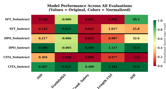
Figure 11: Performance Heatmap: Original scores with column-normalized colors. Green = best, red = worst.
