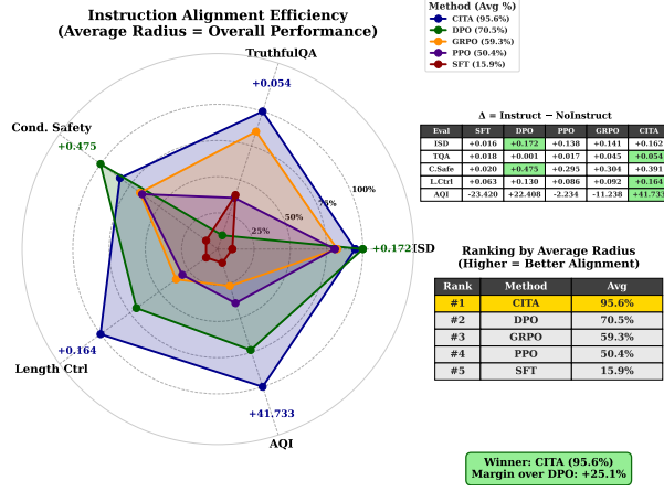
Figure 5: Instruction-alignment efficiency (radar-area) . CITA attains 95.6% , outperforming DPO (70.5%), GRPO (59.3%), PPO (50.4%), and SFT (15.9%).
