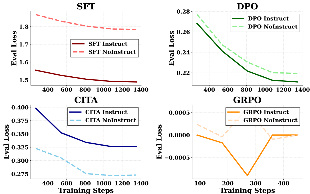
Figure 13: Eval Loss Across Training Methods : 2 \times 2 subplot showing eval loss for all 4 trainer types with independent y-axes (necessary due to vastly different loss scales). SFT (top-left): Loss \sim 1.5 – 1.9 , Instruct converges lower. DPO (top-right): Loss \sim 0.21 – 0.28 , smooth convergence. CITA (bottom-left): Loss \sim 0.27 – 0.40 , NoInstruct converges lower but CITA_Instruct achieves better reward margins. GRPO (bottom-right): Loss oscillates near zero ( \pm 0.001 ), characteristic of online RL training dynamics. Note: PPO tensorboard logs were empty (TRL logging issue).
