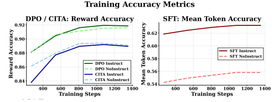
Figure 22: Training Accuracy Metrics: 1 \times 2 subplot comparing accuracy across methods. Left (DPO/CITA): Reward accuracy—all models converge to 89–92%, with DPO variants achieving slightly higher accuracy. Right (SFT): Mean token accuracy—both variants converge smoothly, with Instruct achieving marginally higher accuracy due to richer training signal from instruction-augmented sequences.
