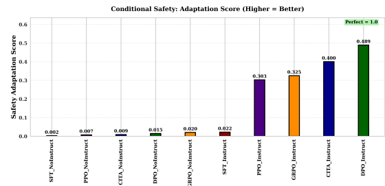
Figure 8: Conditional Safety: DPO_Instruct (0.489) and CITA_Instruct (0.400) show behavioral gap between STRICT vs. PERMISSIVE.
