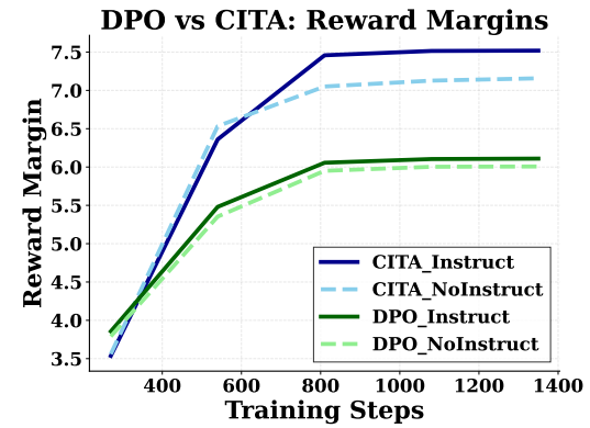
Figure 23: Reward Margins: CITA_Instruct (7.5) > CITA_NoInstruct (7.2) > DPO (~6.0). Higher margins indicate stronger preference learning.
