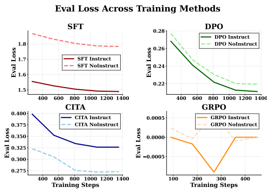
Figure 21: Eval Loss Across Training Methods: 2×2 subplot showing eval loss for all 4 trainer types with independent y-axes (necessary due to vastly different loss scales). SFT (top-left): Loss ~1.5–1.9, Instruct converges lower. DPO (top-right): Loss ~0.21–0.28, smooth convergence. CITA (bottom-left): Loss ~0.27–0.40, NoInstruct converges lower but CITA_Instruct achieves better reward margins. GRPO (bottom-right): Loss oscillates near zero ( \pm 0.001 ), characteristic of online RL training dynamics. Note: PPO tensorboard logs were empty (TRL logging issue).
