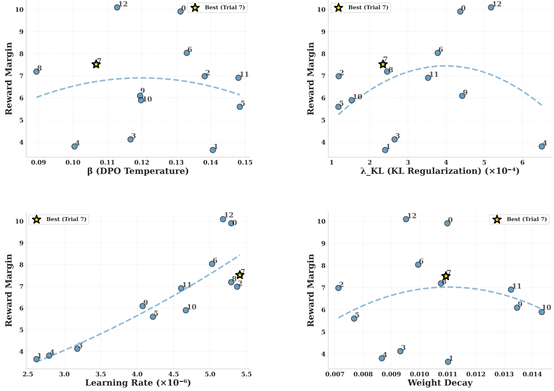
Figure 16: Hyperparameter Ablation Study: Reward margin sensitivity to \beta , \lambda_{KL} , learning rate, and weight decay across 13 Optuna trials. Trial 7 (★) achieves the best trade-off. Key findings: (a) \beta \in [0.10, 0.12] yields highest margins; (b) \lambda_{KL} \approx 0.0002 balances stability and performance; (c) Learning rate sensitivity is high— \sim 5e-6 is optimal for instruction-augmented training; (d) Weight decay shows moderate sensitivity with optimal range \sim 0.01 .
