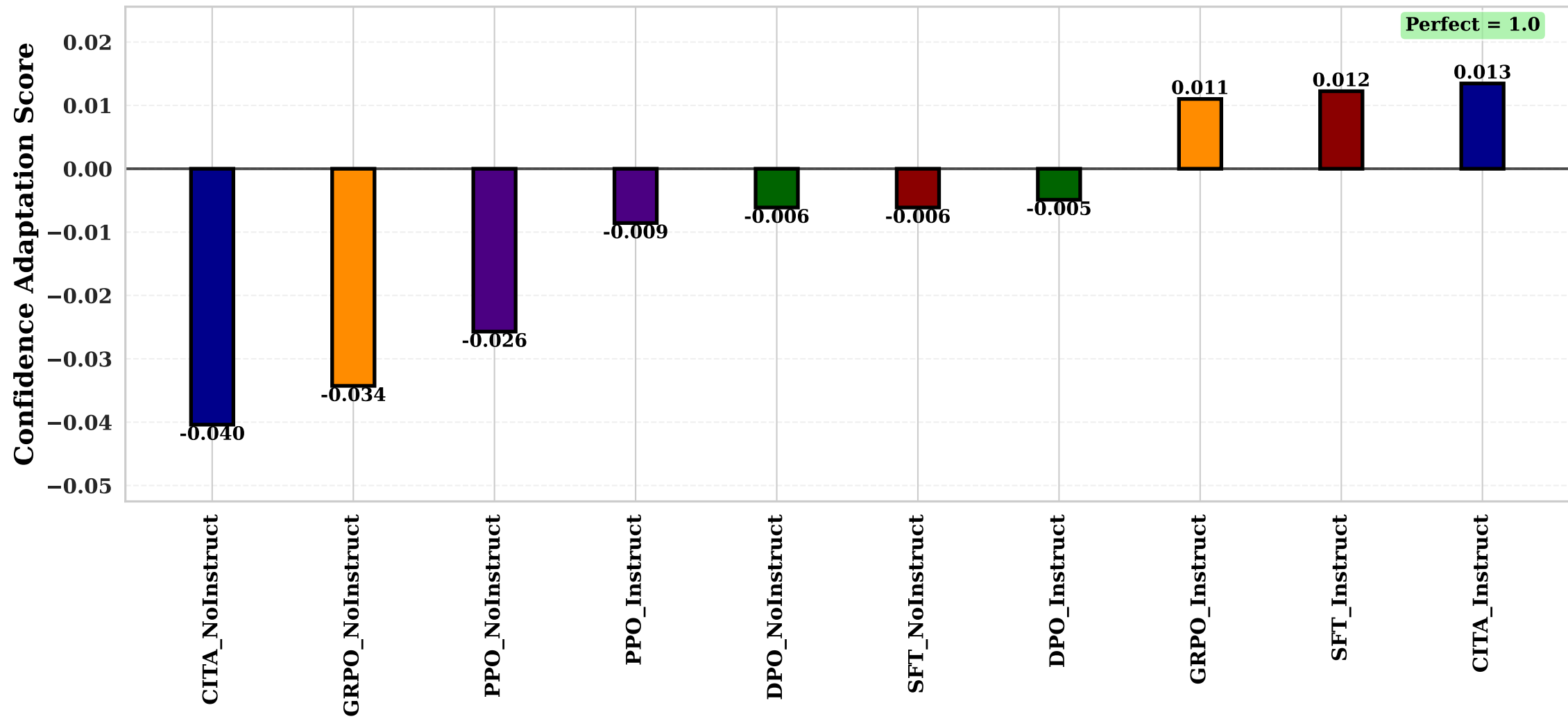
TruthfulQA: Adaptation Score (Positive = Correct)
