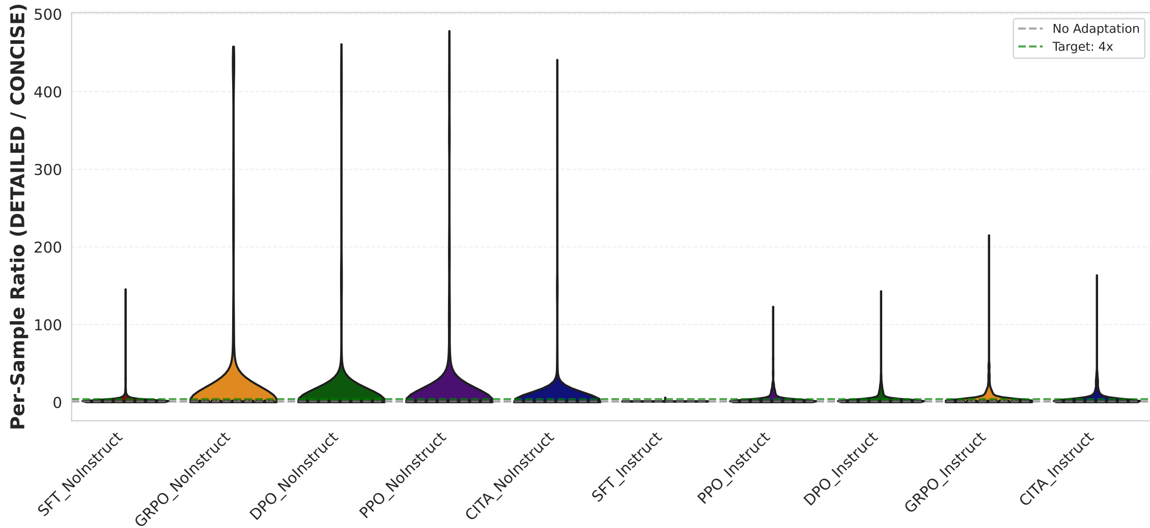
Length Control: Adaptation Ratio Distribution (Violin Plot)
