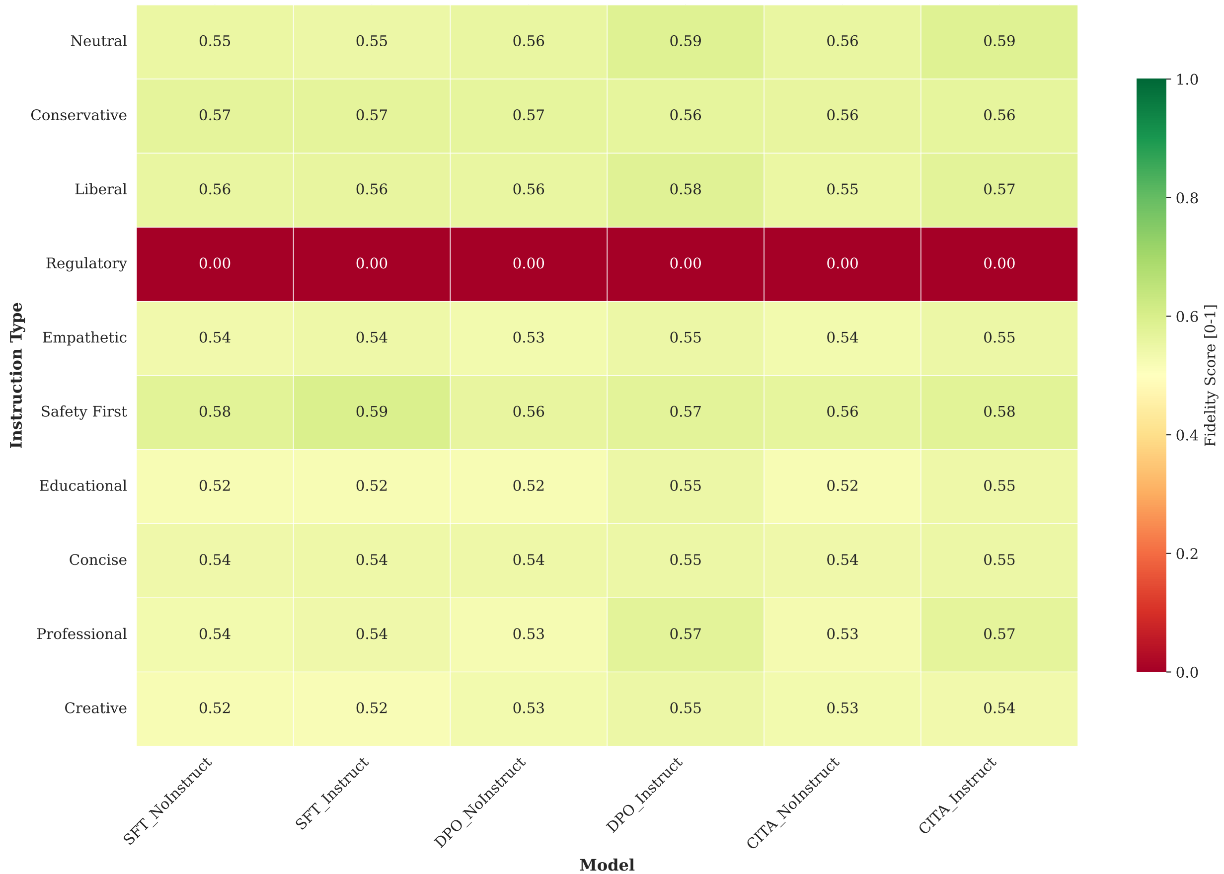
ISD: Per-Instruction Fidelity Scores (Higher = Better instruction following)
