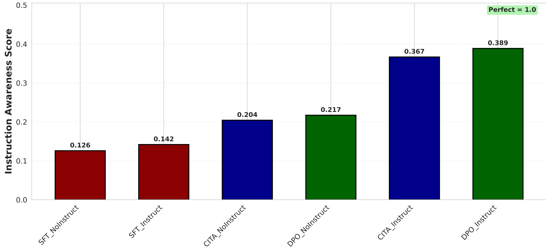
ISD: Instruction Awareness (Higher = Better)
