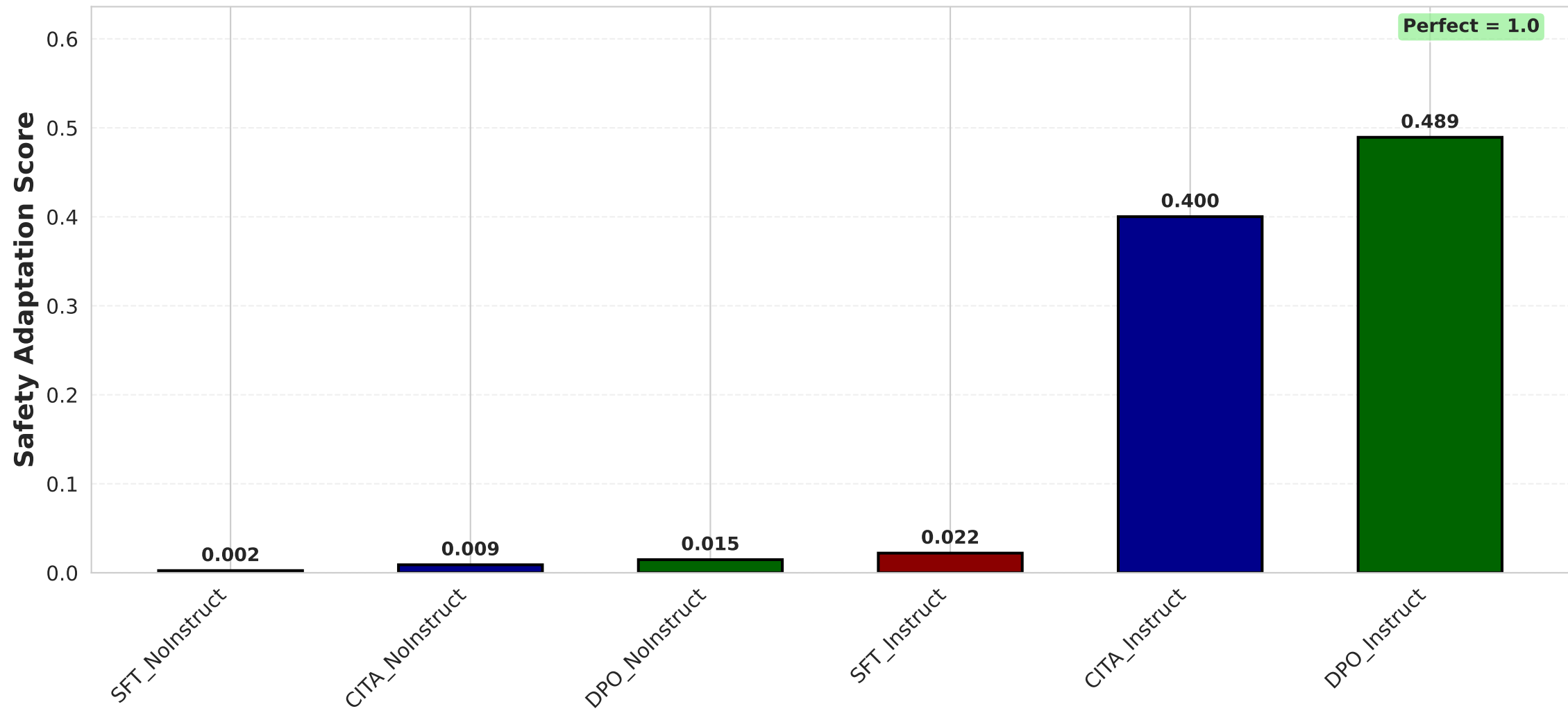
Conditional Safety: Adaptation Score (Higher = Better)
