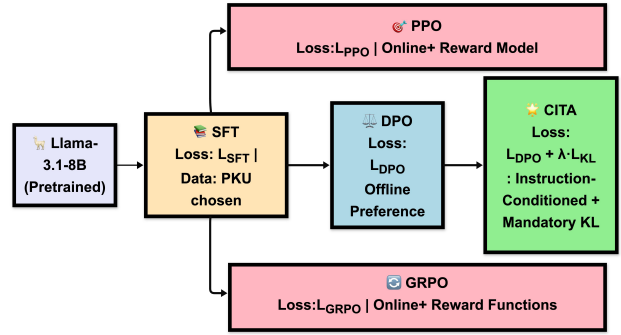
Figure 4. Training pipeline and comparators. All methods branch from SFT. PPO and GRPO are online methods requiring reward models/functions. DPO is an offline preference method. CITA stacks on preference optimization with explicit instruction-conditioning and a mandatory KL anchor .
