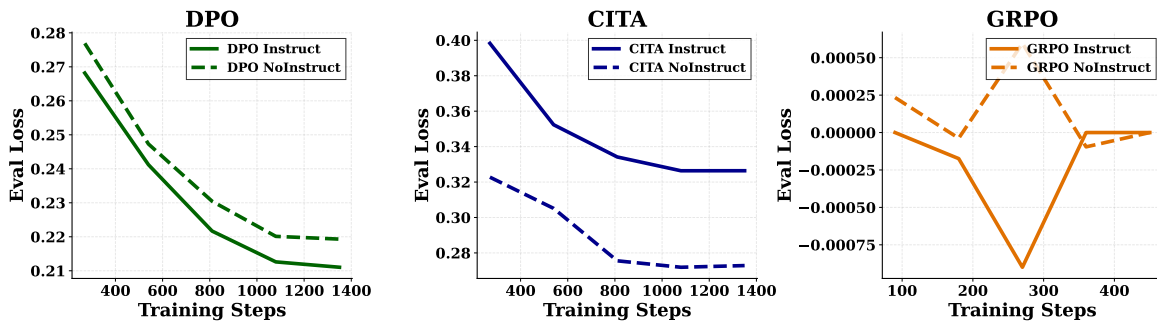
Figure 21. Evaluation loss across policy optimization methods. We plot evaluation loss for DPO, CITA, and GRPO using independent y-axes due to non-comparable loss scales. DPO (left): loss \sim 0.21 – 0.28 with smooth convergence; the Instruct variant is slightly lower, consistent with stronger preference fit under the instruction-augmented setup. CITA (center): loss \sim 0.27 – 0.40 ; the NoInstruct curve converges lower, while CITA_INSTRUCT attains larger reward margins, reflecting a separation–stability trade-off induced by the mandatory anchoring term. GRPO (right): loss oscillates near zero ( \pm 0.001 ), characteristic of online RL training where the objective is dominated by on-policy sampling variance. Note: PPO tensorboard logs were empty due to a TRL logging issue, so we do not include PPO curves here.
