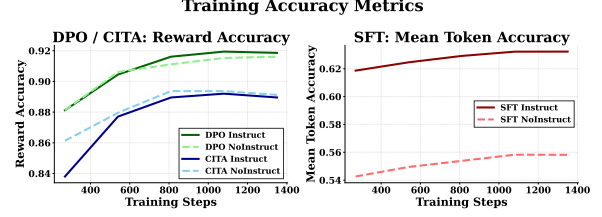
Figure 6: Training Accuracy Metrics: 1 \times 2 subplot comparing accuracy across methods. Left (DPO/CITA): Reward accuracy—all models converge to 89–92%, with DPO variants achieving slightly higher accuracy. Right (SFT): Mean token accuracy—both variants converge smoothly, with Instruct achieving marginally higher accuracy due to richer training signal from instruction-augmented sequences.
