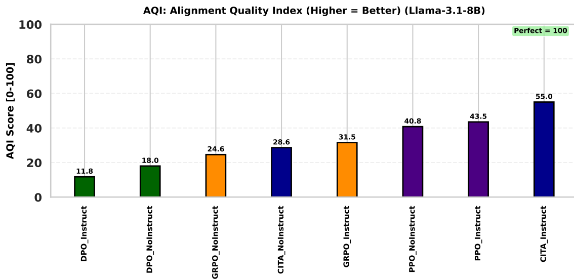
Figure 21: AQI: CITA_Instruct (55.0) achieves highest alignment quality index. PPO variants (40.8–43.5) outperform DPO (11.8–18.0) on cluster separation.
