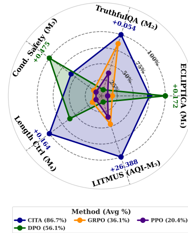
Figure 6: Instruction-alignment efficiency. CITA attains 86.7% , outperforming DPO (56.1%), GRPO (36.1%), and PPO (20.4%). Delta annotations show the winning method’s improvement (Instruct – NoInstruct) per benchmark.
