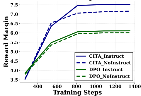
Figure 16: Reward Margins: CITA_Instruct (7.5) > CITA_NoInstruct (7.2) > DPO (~6.0). Higher margins indicate stronger preference learning.
