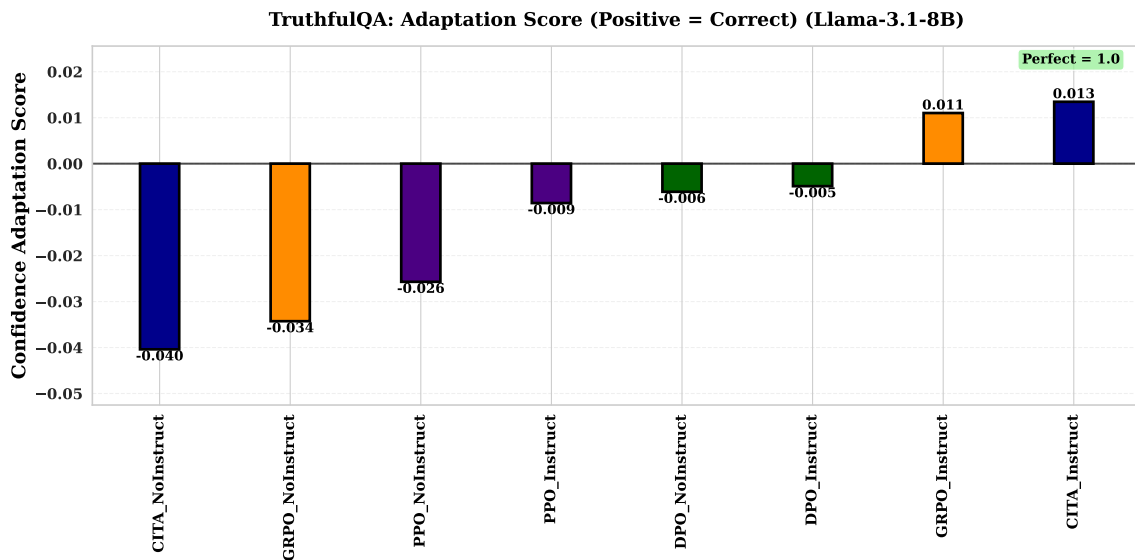
Figure 18: TruthfulQA: Only CITA_Instruct (+0.013) and GRPO_Instruct (+0.011) achieve positive adaptation scores, indicating improved confidence calibration.
