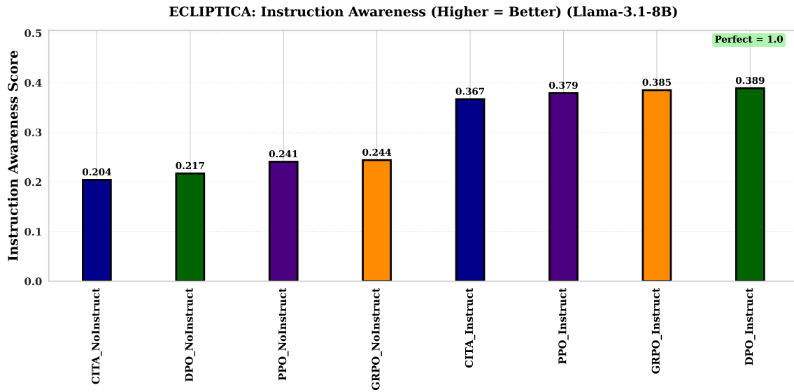
Figure 17: ECLIPTICA Results: DPO_Instruct (0.389) and CITA_Instruct (0.367) show highest instruction awareness.
