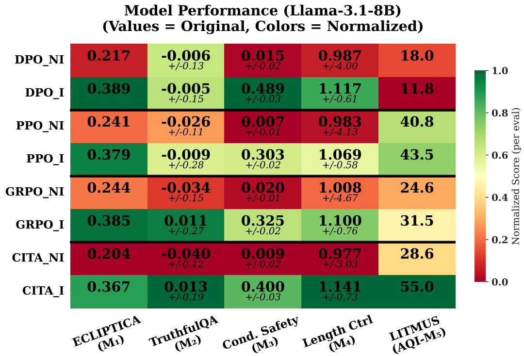
Figure 22: Performance Heatmap with Bootstrap Confidence Intervals (CI) : Original scores (bold) with 95% CI (italic, \pm ) for 3/5 benchmarks. Colors are column-normalized (green = best, red = worst). CI computed via 1,000 bootstrap resamples from per-sample metrics: TruthfulQA (binary uncertainty difference), Cond. Safety (binary refusal difference), Length Ctrl (ratio of means). ECLIPTICA and AQI lack per-sample decomposition (composite/cluster-based metrics).
