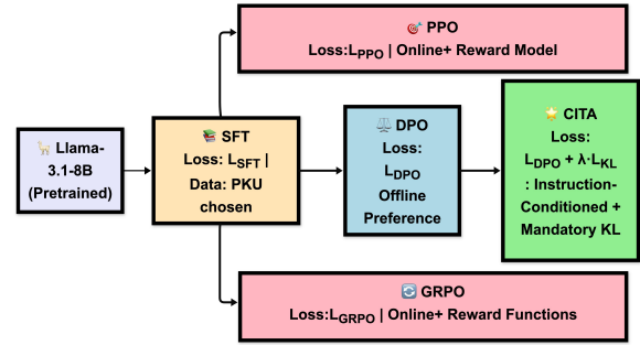
Figure 4: All methods branch from SFT. PPO and GRPO are online methods requiring reward model/functions. DPO uses offline preference pairs. CITA stacks on DPO with instruction-conditioning.
