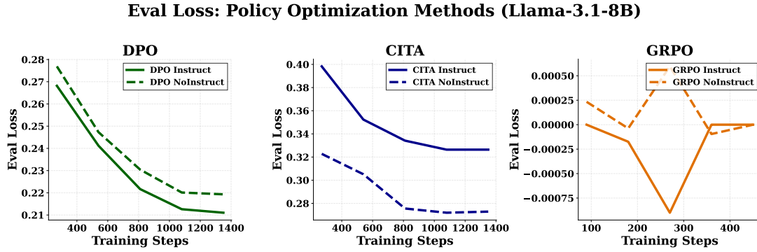
Figure 14: Eval Loss Across Policy Optimization Methods: 1 \times 3 subplot showing eval loss for DPO, CITA, and GRPO with independent y-axes (necessary due to vastly different loss scales). DPO (left): Loss \sim 0.21 – 0.28 , smooth convergence with Instruct slightly lower. CITA (center): Loss \sim 0.27 – 0.40 , NoInstruct converges lower but CITA_Instruct achieves better reward margins. GRPO (right): Loss oscillates near zero ( \pm 0.001 ), characteristic of online RL training dynamics. Note: PPO tensorboard logs were empty (TRL logging issue).
