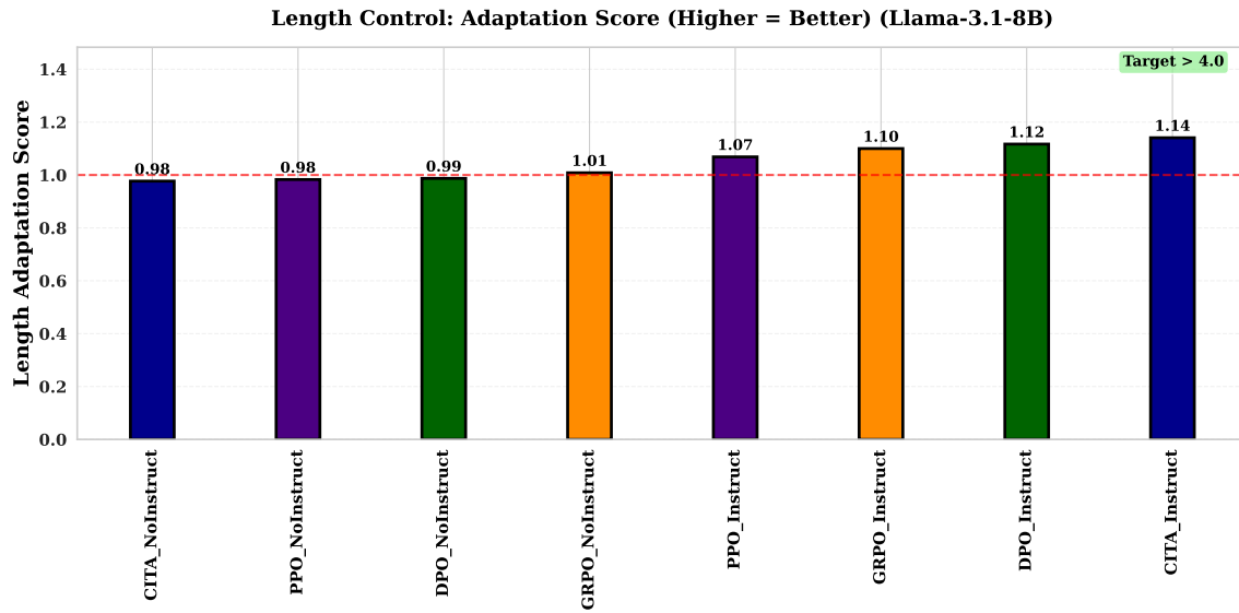
Figure 20: Length Control: CITA_Instruct (1.14) shows strongest adaptation ratio (detailed/concise word count).
