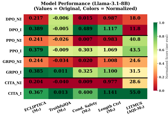
Figure 7: Performance heatmap across 5 benchmarks. Original scores with column-normalized colors (green = best, red = worst per column). NI = NoInstruct, I = Instruct. CITA_I achieves highest AQI (55.0) and competitive performance across all metrics.
