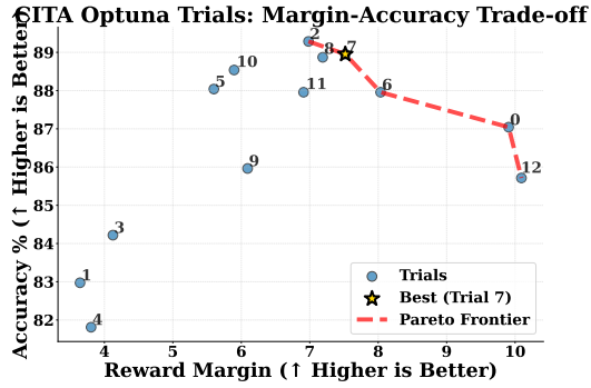
Figure 15: Pareto Frontier: Margin vs. accuracy trade-off across trials. Trial 7 lies on the Pareto frontier, achieving near-optimal balance (margin=7.52, accuracy=89%).
