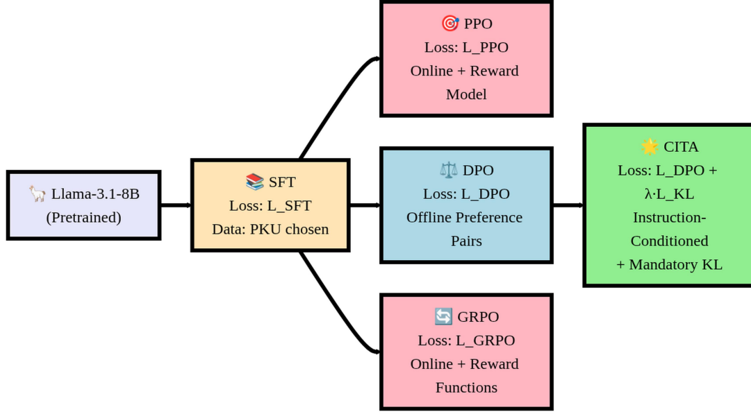
Figure 3: Training Pipeline: All methods branch from SFT. PPO and GRPO are online methods requiring reward model/functions. DPO uses offline preference pairs. CITA stacks on DPO with instruction-conditioning and mandatory KL regularization.
