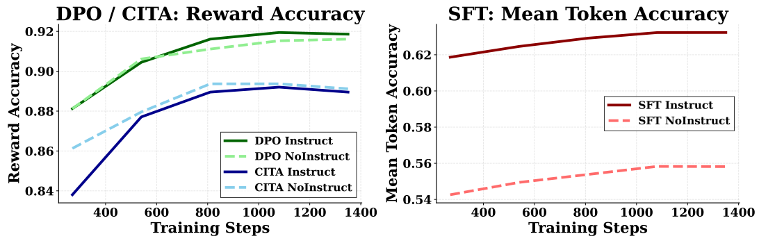
Figure 5: Training Accuracy Metrics: 1 \times 2 subplot comparing accuracy across methods. Left (DPO/CITA): Reward accuracy—all models converge to 89–92%, with DPO variants achieving slightly higher accuracy. Right (SFT): Mean token accuracy—both variants converge smoothly, with Instruct achieving marginally higher accuracy due to richer training signal from instruction-augmented sequences.
