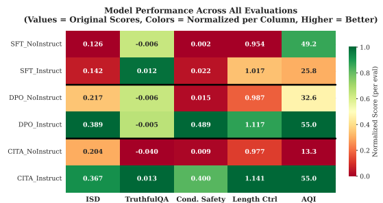
Figure 13: Performance Heatmap: Original scores with column-normalized colors. Green = best, red = worst.
