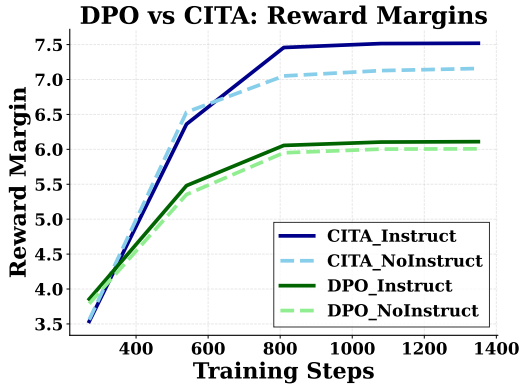
Figure 6: Reward Margins: CITA_Instruct (7.5) > CITA_NoInstruct (7.1) > DPO (~6.0). Higher margins indicate stronger preference learning.
