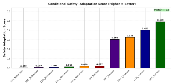
Figure 9: Conditional Safety: DPO_Instruct (0.489) and CITA_Instruct (0.400) show behavioral gap between STRICT vs. PERMISSIVE.
