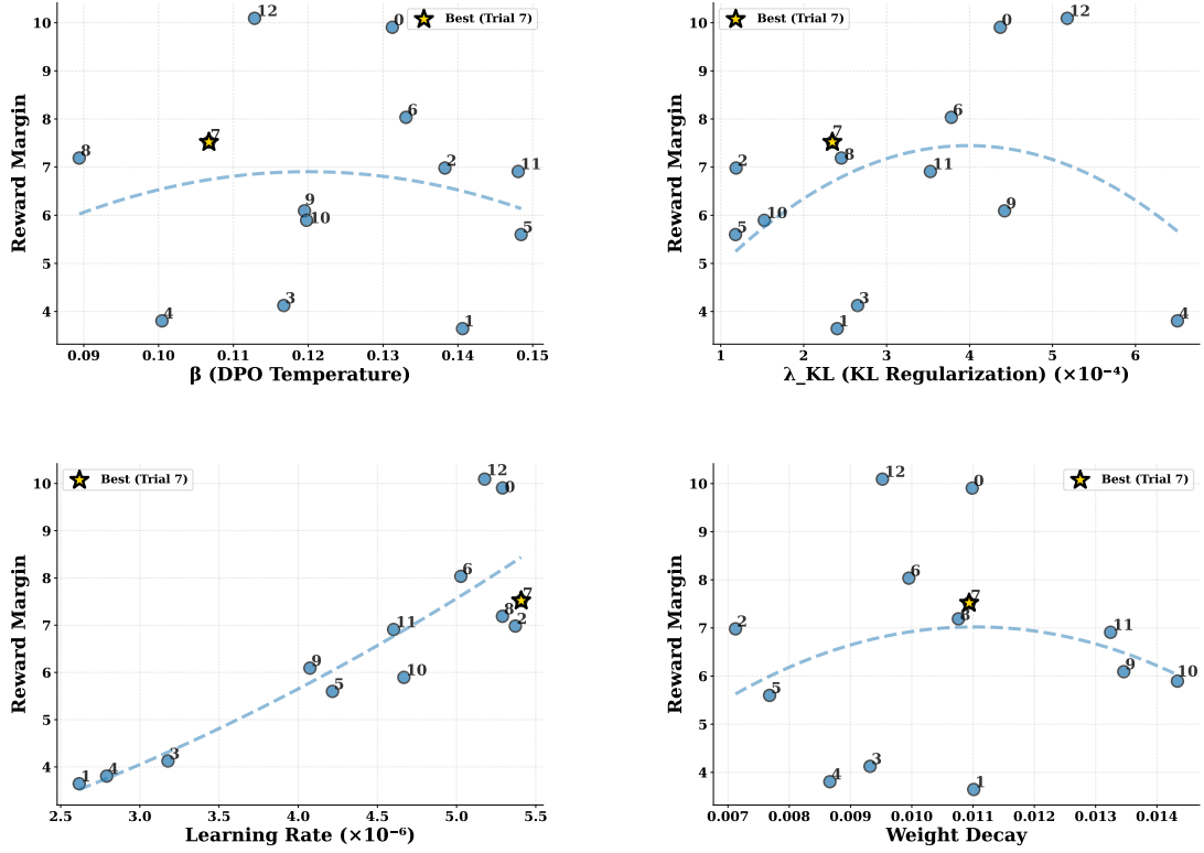
Figure 14: Hyperparameter Ablation Study: Reward margin sensitivity to \beta , \lambda_{KL} , learning rate, and weight decay across 13 Optuna trials. Trial 7 (★) achieves the best trade-off. Key findings: (a) \beta \in [0.10, 0.12] yields highest margins; (b) \lambda_{KL} \approx 0.0002 balances stability and performance; (c) Learning rate sensitivity is high— \sim 5\text{e-}6 is optimal for instruction-augmented training; (d) Weight decay shows moderate sensitivity with optimal range \sim 0.01 .
