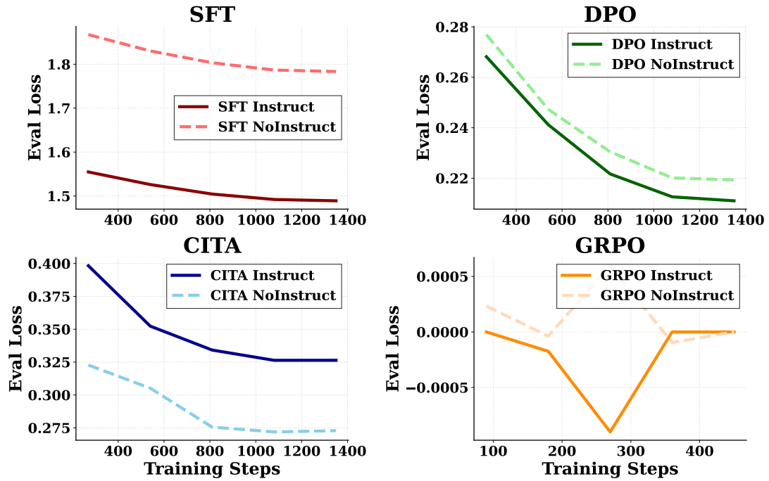
Figure 4: Eval Loss Across Training Methods: 2×2 subplot showing eval loss for all 4 trainer types with independent y-axes (necessary due to vastly different loss scales). SFT (top-left): Loss ~1.5–1.9, Instruct converges lower. DPO (top-right): Loss ~0.21–0.28, smooth convergence. CITA (bottom-left): Loss ~0.27–0.40, NoInstruct converges lower but CITA_Instruct achieves better reward margins. GRPO (bottom-right): Loss oscillates near zero ( \pm 0.001 ), characteristic of online RL training dynamics. Note: PPO tensorboard logs were empty (TRL logging issue).
