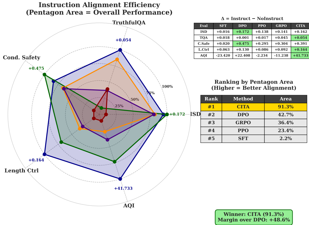
Figure 12: Instruction Alignment Efficiency: Pentagon area represents overall performance. CITA achieves 91.3% area (rank #1), outperforming DPO (42.7%), GRPO (36.4%), PPO (23.4%), and SFT (2.2%). CITA wins 3/5 benchmarks with +48.6% margin over DPO.
