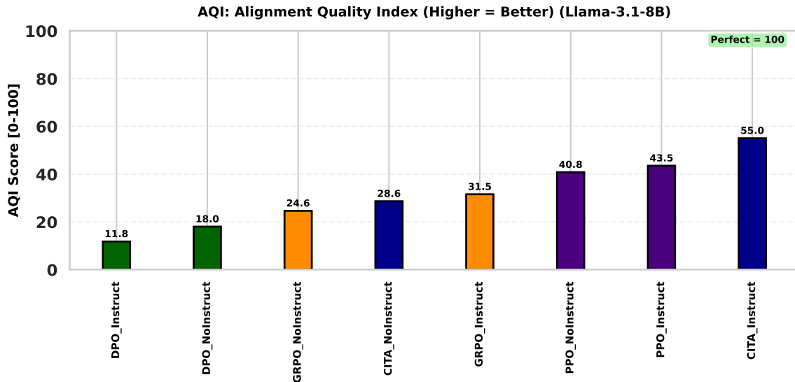
Figure 21: AQI . CITA_Instruct (55.0) achieves the highest AQI. PPO variants (40.8–43.5) outperform DPO (11.8–18.0) on cluster separation.
