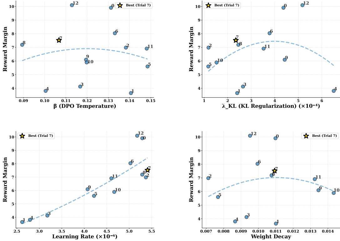
Figure 9: Hyperparameter sensitivity across 13 Optuna trials. Reward margin is most sensitive to learning rate and the (\beta, \lambda_{KL}) interaction. Trial 7 ( \star ) achieves the best trade-off, aligning with the “Goldilocks” band: \beta \in [0.10, 0.12] , \lambda_{KL} \approx 2 \times 10^{-4} , and LR \approx 5 \times 10^{-6} .
