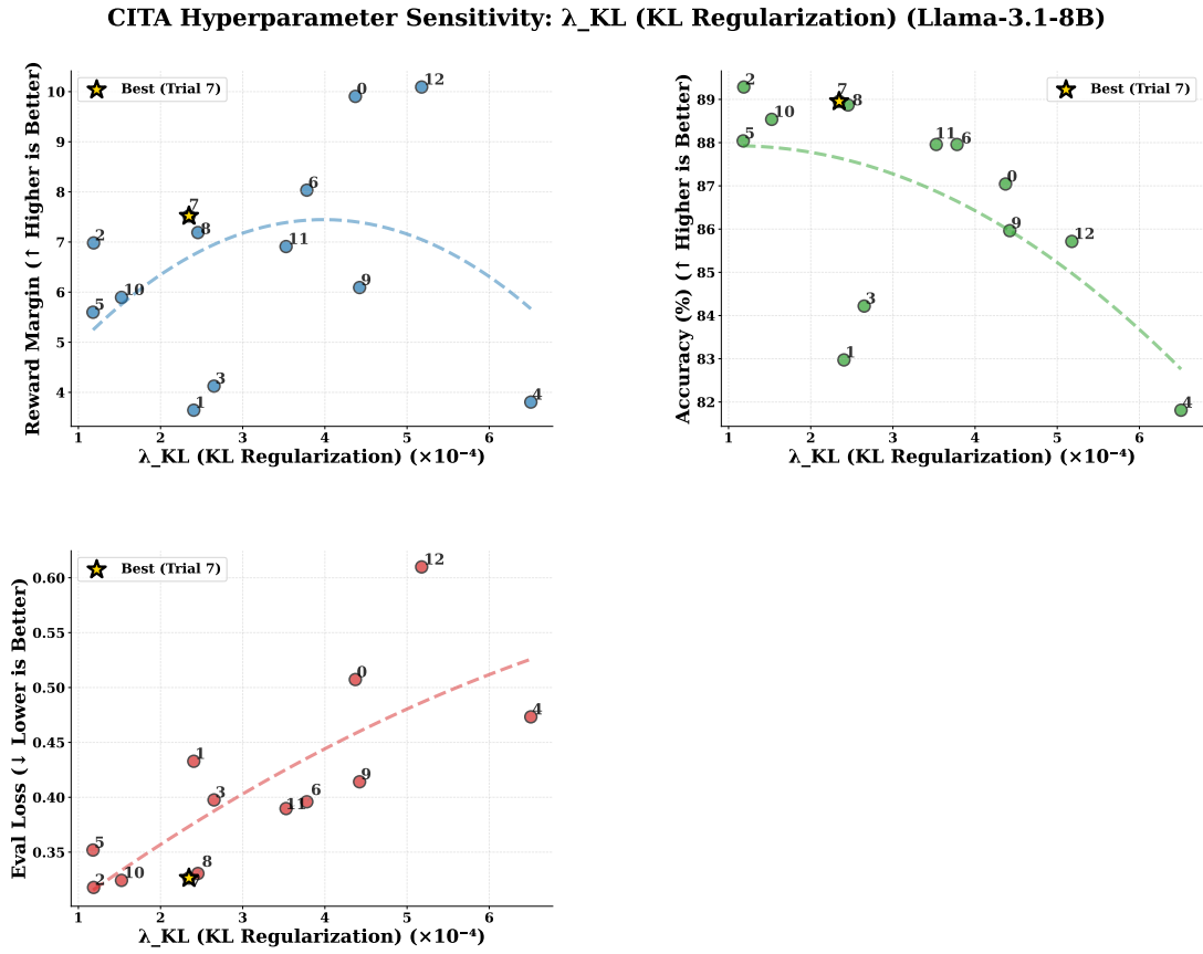
Figure 12: \lambda_{KL} sensitivity . Reward margin exhibits an inverted-U: too low produces instability and regime interference; too high suppresses learning. Accuracy is comparatively stable, indicating the dominant effect is on switching stability rather than raw preference fit. Trial 7 ( \star ) at \lambda_{KL}=0.00023 lies in the optimal band.
