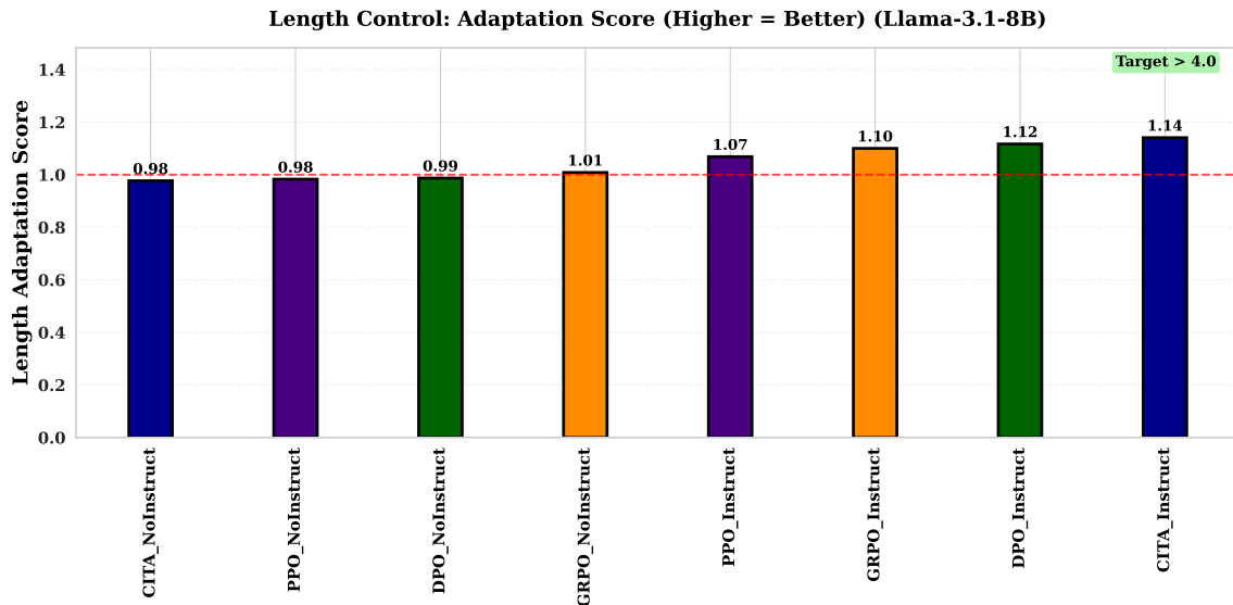
Figure 20: Length control. CITA_Instruct (1.14) shows the strongest adaptation ratio (detailed/concise word count), indicating reliable compliance with explicit verbosity contracts.
