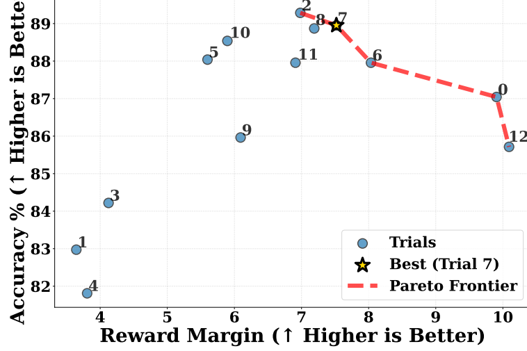
Figure 10: Pareto frontier across trials. Trial 7 lies on the frontier, achieving near-optimal balance (margin=7.52, accuracy=89%) while maintaining strong instruction-conditioned switching.
