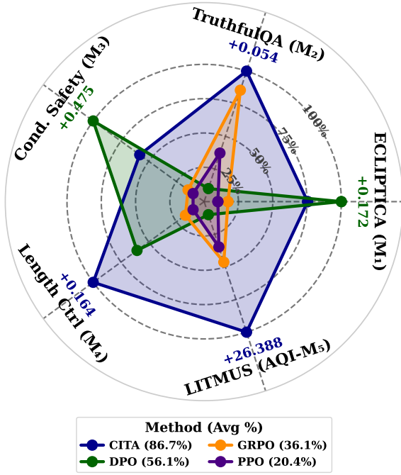
Figure 6: Instruction-alignment efficiency. CITA achieves 86.7% , outperforming DPO (56.1%), GRPO (36.1%), and PPO (20.4%).
