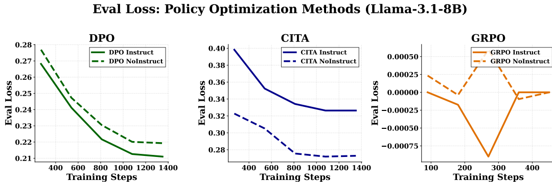
Figure 14: Evaluation loss across policy optimization methods. We plot evaluation loss for DPO, CITA, and GRPO using independent y-axes due to non-comparable loss scales. DPO (left): loss \sim 0.21 – 0.28 with smooth convergence; the Instruct variant is slightly lower, consistent with stronger preference fit under the instruction-augmented setup. CITA (center): loss \sim 0.27 – 0.40 ; the NoInstruct curve converges lower, while CITA_INSTRUCT attains larger reward margins, reflecting a separation–stability trade-off induced by the mandatory anchoring term. GRPO (right): loss oscillates near zero ( \pm 0.001 ), characteristic of online RL training where the objective is dominated by on-policy sampling variance. Note: PPO tensorboard logs were empty due to a TRL logging issue, so we do not include PPO curves here.
