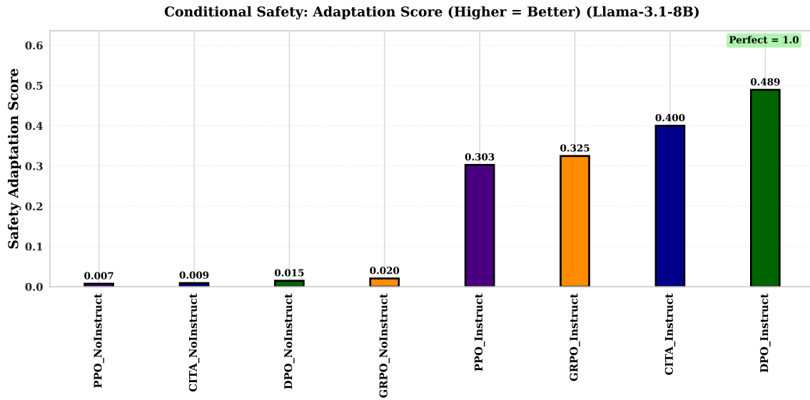
Figure 19: Conditional Safety. DPO_Instruct (0.489) and CITA_Instruct (0.400) show the strongest behavioral gap between STRICT vs. PERMISSIVE instructions.
