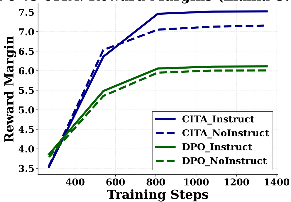
Figure 16: Reward margins. CITA_Instruct (7.5) > CITA_NoInstruct (7.2) > DPO (~6.0). Larger margins indicate stronger separation between preferred vs. dispreferred responses under the instruction-conditioned preference relation.
