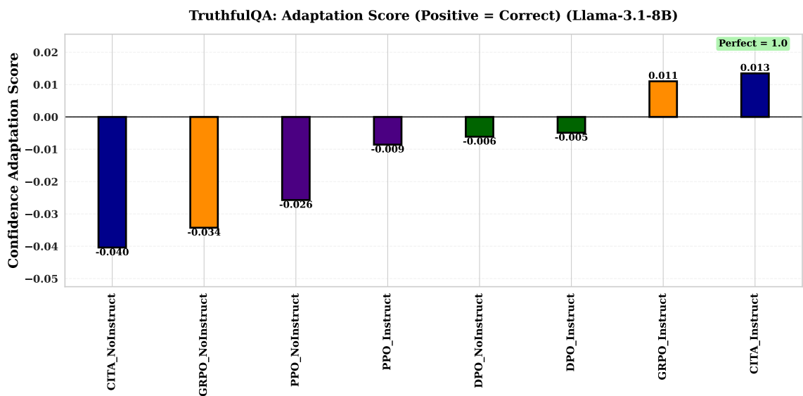
Figure 18: TruthfulQA . Only CITA_Instruct (+0.013) and GRPO_Instruct (+0.011) achieve positive adaptation scores, indicating improved confidence calibration under instruction.
