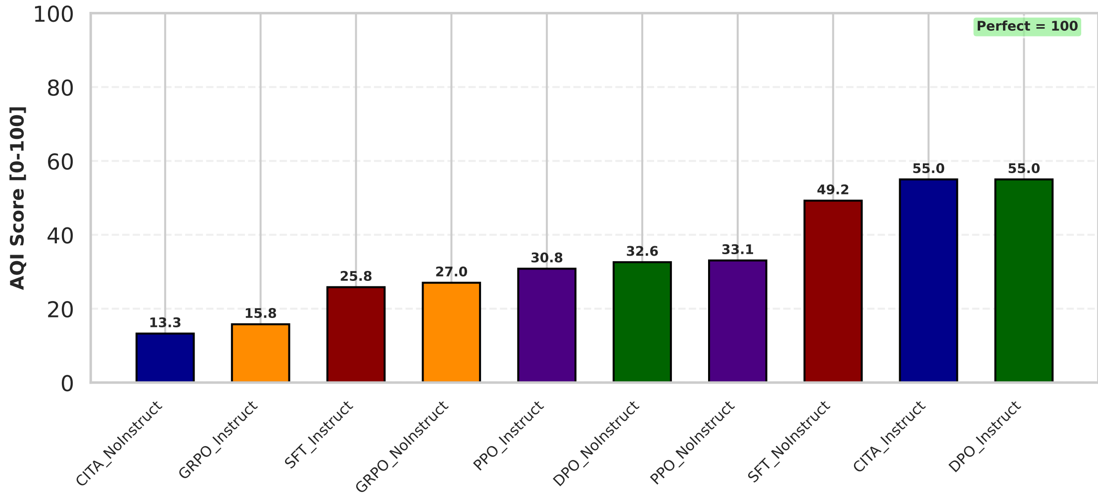
AQI: Alignment Quality Index (Higher = Better)
