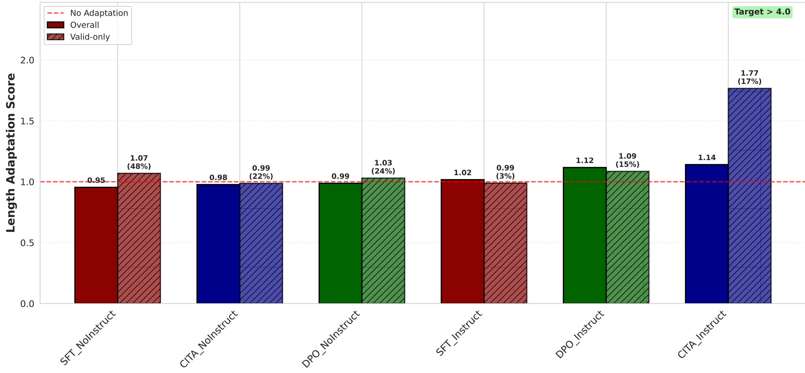
Length Control: Adaptation Score - Overall vs Valid-Only (Higher = Better)
