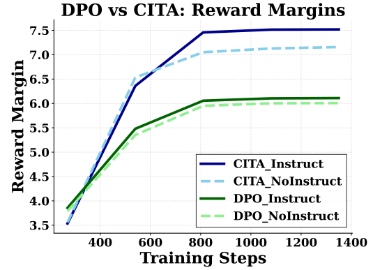
Figure 4: Reward Margins: CITA_Instruct (7.5) > CITA_NoInstruct (7.2) > DPO (~6.0). Higher margins indicate stronger preference learning.
