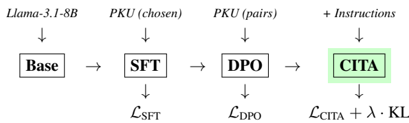
Figure 2: CITA training pipeline. Each stage uses the previous checkpoint. CITA adds mandatory KL regularization for instruction-conditioned alignment.
