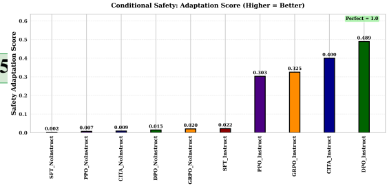
Figure 9: Conditional Safety : DPO_Instruct (0.489) and CITA_Instruct (0.400) show behavioral gap between STRICT vs. PERMISSIVE.
