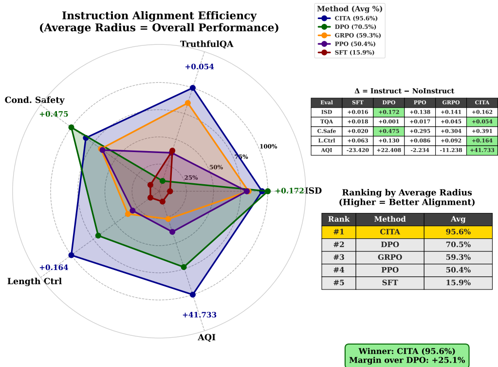
Figure 12: Instruction Alignment Efficiency : Average normalized radius represents overall instruction-alignment performance (see Eq. (14)). CITA achieves 95.6% —outperforming DPO (70.5%) by 25.1 pp, GRPO (59.3%) by 36.3 pp, PPO (50.4%) by 45.2 pp, and SFT (15.9%) by 79.7 pp.
