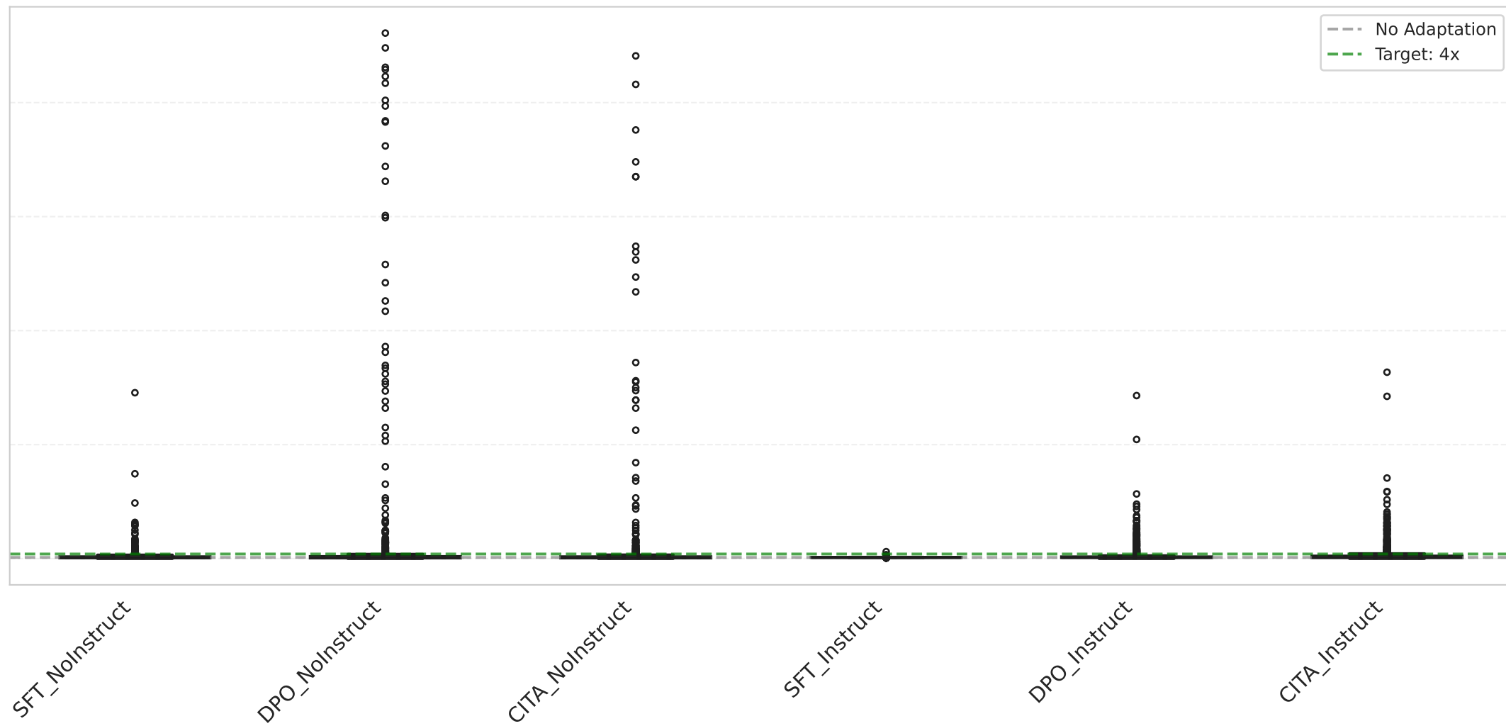
Length Control: Adaptation Ratio Distribution (Box Plot)
