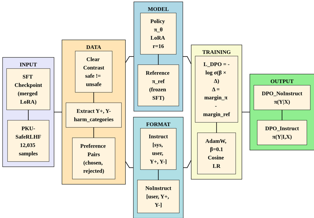
Figure 24: DPO Training Pipeline. Starting from a merged SFT checkpoint (LoRA adapters merged into base weights), the pipeline creates two models: a trainable Policy \pi_\theta with fresh LoRA adapters ( r=16 ) and a frozen Reference \pi_{ref} (exact copy of merged SFT). PKU-SafeRLHF data undergoes clear contrast filtering ( \text{is\_response\_0\_safe} \neq \text{is\_response\_1\_safe} ) to extract preference pairs ( Y^+, Y^- ) and harm categories. For the Instruct variant, alignment instructions are synthesized from harm categories and formatted as [sys, user, chosen, rejected]; for NoInstruct , the format is [user, chosen, rejected]. Training uses DPO loss: \mathcal{L}_{DPO} = -\log \sigma(\beta \cdot \Delta) where \Delta = \text{margin}_\pi - \text{margin}_{ref} and \beta = 0.1 . Output: two trained policies \pi_{DPO\_NoInstruct}(Y|X) and \pi_{DPO\_Instruct}(Y|I, X) .
