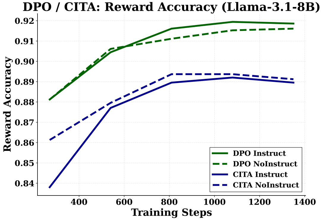
Figure 15: Training accuracy metrics. Reward accuracy for DPO/CITA variants. All converge to \sim 89\text{--}92\% , with DPO slightly higher.
