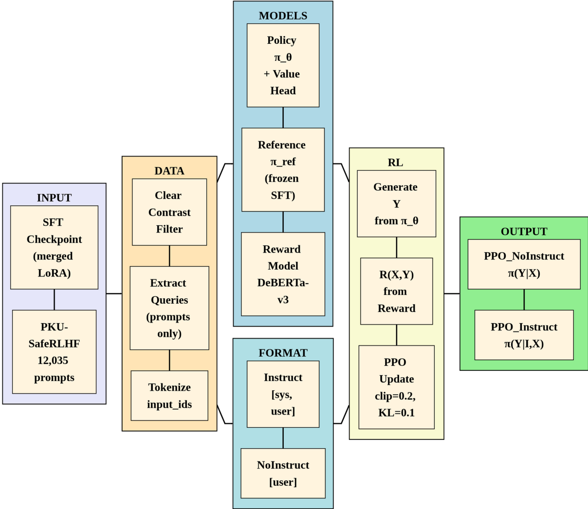
Figure 25: PPO Training Pipeline . Starting from a merged SFT checkpoint , PPO maintains three models : (1) trainable Policy \pi_\theta with a value head for advantage estimation, (2) frozen Reference \pi_{\text{ref}} for KL regularization, and (3) external Reward Model (OpenAssistant DeBERTa-v3-large). Unlike DPO, PPO only requires queries (prompts)—not preference pairs—from PKU-SafeRLHF. The online RL loop iterates: (i) generate responses Y from policy, (ii) score with reward model R(X, Y) , (iii) compute GAE advantage ( \gamma = 1.0 , \lambda = 0.95 ), (iv) PPO update with clipped surrogate objective ( \epsilon = 0.2 ) and KL penalty (coef= 0.1). Output: \pi_{\text{PPO\_NoInstruct}}(Y|X) and \pi_{\text{PPO\_Instruct}}(Y|I, X) .
