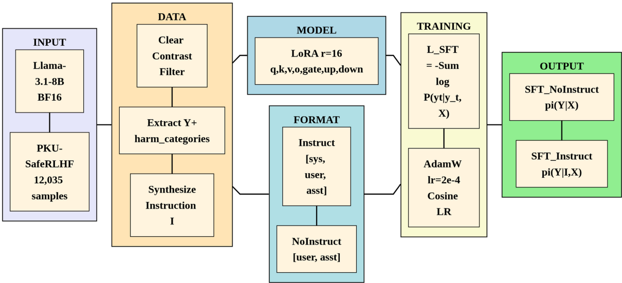
Figure 23: SFT Training Pipeline. Starting from Llama-3.1-8B (BF16) and PKU-SafeRLHF dataset (12,035 samples), the pipeline applies clear contrast filtering to extract safe responses ( Y^+ ) and harm categories. For the Instruct variant, alignment instructions are synthesized from harm categories and formatted as [sys, user, asst]; for NoInstruct , the format is [user, asst]. LoRA adapters ( r=16 ) target attention and MLP projections. Training uses cross-entropy loss with AdamW optimizer ( lr=2e-4 ) and cosine LR schedule, producing two trained policies: \pi_{\text{SFT\_NoInstruct}}(Y|X) and \pi_{\text{SFT\_Instruct}}(Y|I, X) .
