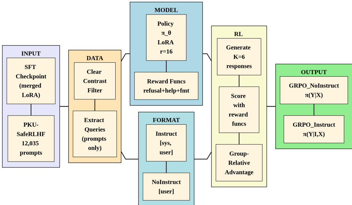
Figure 26: GRPO Training Pipeline . Unlike PPO, GRPO requires no reference model —advantages are computed group-relative within each batch. Starting from a merged SFT checkpoint, the policy \pi_\theta generates K = 6 responses per prompt. Reward functions (heuristic): (i) safety_refusal (+1.0 for refusing harmful requests), (ii) helpfulness (+1.0 for substantive responses), (iii) format_quality (+0.5 for proper structure). The group-relative advantage normalizes rewards within the batch: \hat{A}(y_i) = (R(y_i) - \mu_{\text{batch}}) / \sigma_{\text{batch}} , enabling policy gradient updates without KL regularization. Output: \pi_{\text{GRPO\_NoInstruct}}(Y|X) and \pi_{\text{GRPO\_Instruct}}(Y|I, X) .
