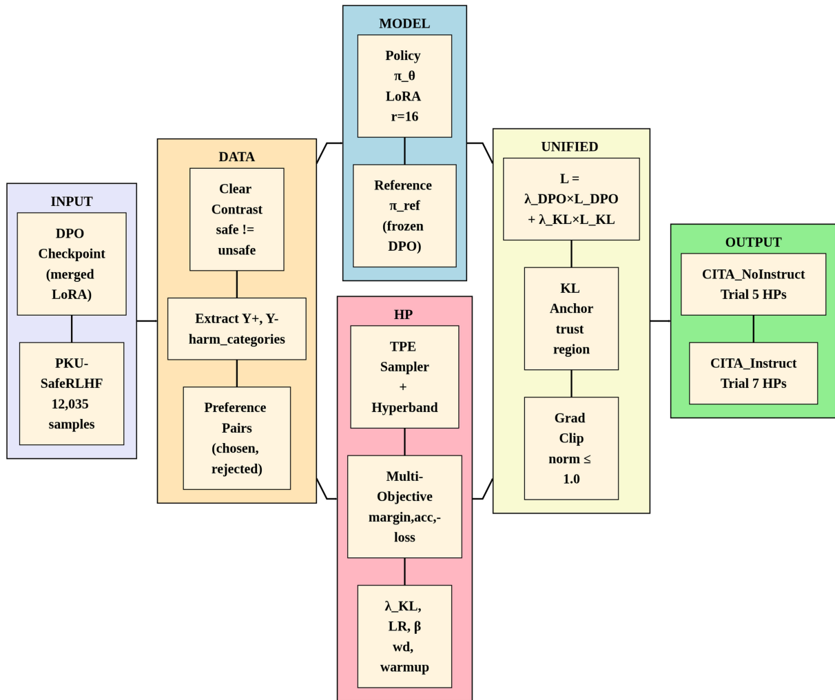
Figure 27: CITA Training Pipeline. CITA stacks on DPO (not SFT) and adds a mandatory KL anchor for stable multi-regime switching. Unified loss: \mathcal{L}_{CITA} = \lambda_{DPO} \cdot \mathcal{L}_{DPO} + \lambda_{KL} \cdot \mathcal{L}_{KL} , where \mathcal{L}_{KL} = \frac{1}{2}[\text{mean}(\log \pi_\theta - \log \pi_{ref})_{\text{chosen}} + \text{mean}(\log \pi_\theta - \log \pi_{ref})_{\text{rejected}}] . NO \mathcal{L}_{SFT} —adding SFT loss causes catastrophic interference on DPO-tuned models (margin collapse 2.95 \rightarrow 0.10 ). Hyperparameter tuning: Optuna TPE sampler with Hyperband pruner optimizes ( \lambda_{KL} , LR, \beta , weight_decay, warmup_ratio) via multi-objective optimization (maximize margin, accuracy; minimize eval_loss). Instruct variant uses \sim 50\% lower LR due to longer sequences (30–40% more tokens). Final models use Trial 5 HPs (NoInstruct: margin=6.95) and Trial 7 HPs (Instruct: margin=7.52). Gradient clipping ( \|\nabla\| \leq 1.0 ) prevents training explosion. Output: \pi_{CITA\_NoInstruct}(Y|X) and \pi_{CITA\_Instruct}(Y|I, X) .
