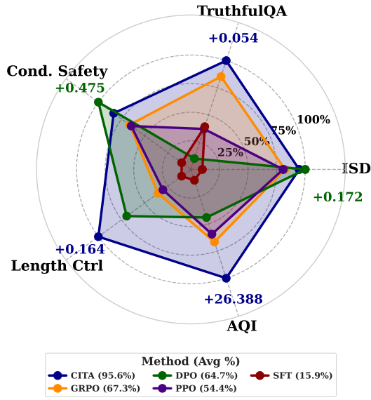
Figure 8: Instruction-alignment efficiency (radar-area) . CITA attains 95.6% , outperforming DPO (64.7%), GRPO (67.3%), PPO (54.4%), and SFT (15.9%). Delta annotations show the winning method’s improvement (Instruct – NoInstruct) per benchmark.
