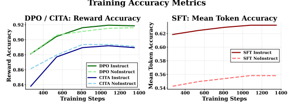
Figure 6: Training Accuracy Metrics : 1 \times 2 subplot comparing accuracy across methods. Left (DPO/CITA) : Reward accuracy—all models converge to 89–92%, with DPO variants achieving slightly higher accuracy. Right (SFT) : Mean token accuracy—both variants converge smoothly, with Instruct achieving marginally higher accuracy due to richer training signal from instruction-augmented sequences.
