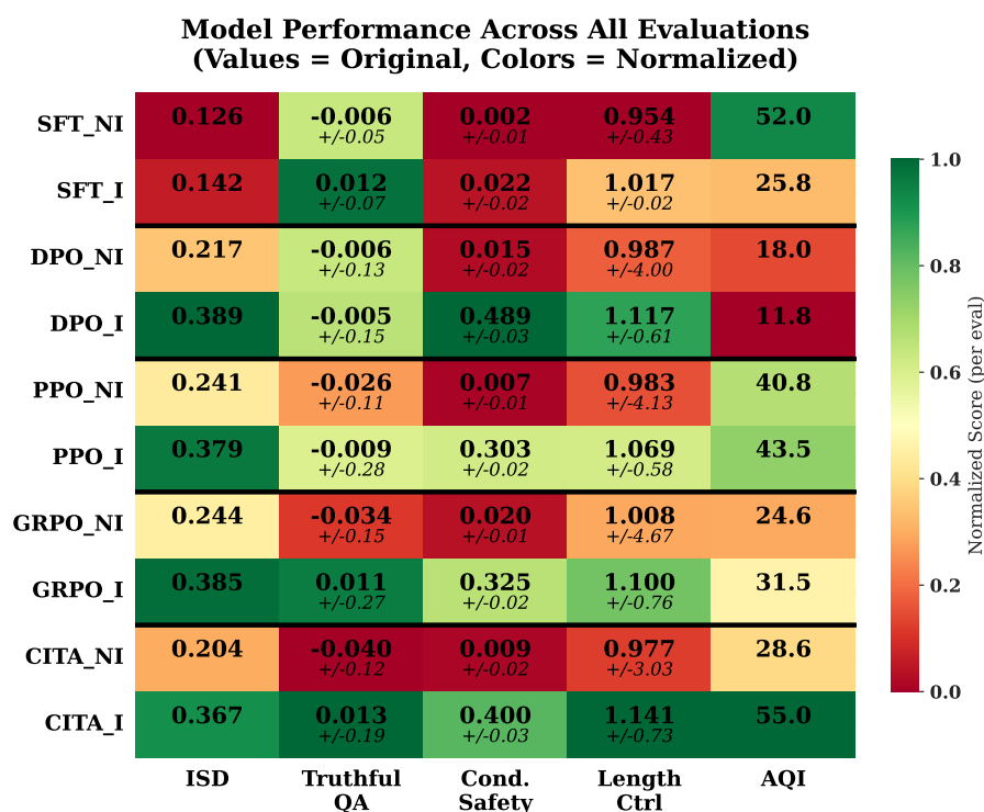
Figure 15: Performance Heatmap with Bootstrap Confidence Intervals (CI) : Original scores (bold) with 95% CI (italic, \pm ) for 3/5 benchmarks. Colors are column-normalized (green = best, red = worst). CI computed via 1,000 bootstrap resamples from per-sample metrics: TruthfulQA (binary uncertainty difference), Cond. Safety (binary refusal difference), Length Ctrl (ratio of means). ISD and AQI lack per-sample decomposition (composite/cluster-based metrics).
