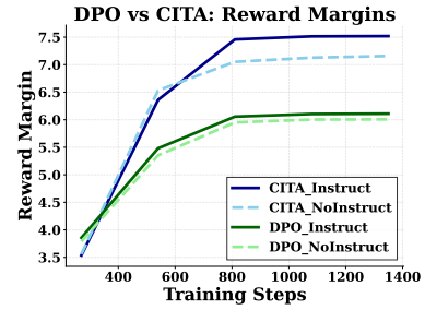
Figure 7: Reward Margins : CITA_Instruct (7.5) > CITA_NoInstruct (7.2) > DPO ( \sim 6.0 ). Higher margins indicate stronger preference learning.
