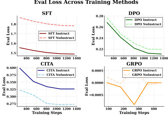
Figure 5: Eval Loss Across Training Methods : 2 \times 2 subplot showing eval loss for all 4 trainer types with independent y-axes (necessary due to vastly different loss scales). SFT (top-left): Loss \sim 1.5 – 1.9 , Instruct converges lower. DPO (top-right): Loss \sim 0.21 – 0.28 , smooth convergence. CITA (bottom-left): Loss \sim 0.27 – 0.40 , NoInstruct converges lower but CITA_Instruct achieves better reward margins. GRPO (bottom-right): Loss oscillates near zero ( \pm 0.001 ), characteristic of online RL training dynamics. Note: PPO tensorboard logs were empty (TRL logging issue).
