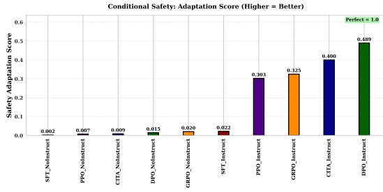
Figure 12: Conditional Safety: DPO_Instruct (0.489) and CITA_Instruct (0.400) show behavioral gap between STRICT vs. PERMISSIVE.
