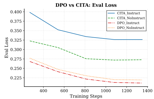
Figure 16: Eval Loss: CITA_Instruct has higher loss but achieves better reward margins (see Figure ??). This apparent paradox is explained by CITA’s mandatory KL regularization, which prevents over-optimization on the training distribution while maintaining stronger preference separation.
