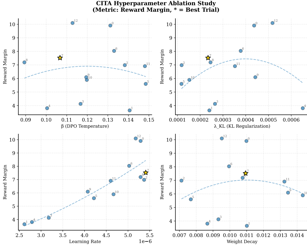
Figure 11: Hyperparameter Ablation Study: Reward margin sensitivity to \beta , \lambda_{KL} , learning rate, and weight decay across 13 Optuna trials. Trial 7 (★) achieves the best trade-off. Key findings: (a) \beta \in [0.10, 0.12] yields highest margins; (b) \lambda_{KL} \approx 0.0002 balances stability and performance; (c) Learning rate sensitivity is high— \sim 5e-6 is optimal for instruction-augmented training; (d) Weight decay shows moderate sensitivity with optimal range \sim 0.01 .
