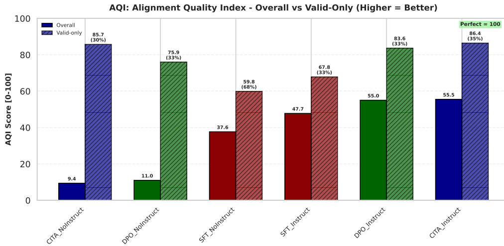
Figure 8: AQI (Alignment Quality Index): CITA_Instruct (55.5) and DPO_Instruct (55.0) achieve highest clustering scores. Valid-only scores (hatched) reach 86%.
