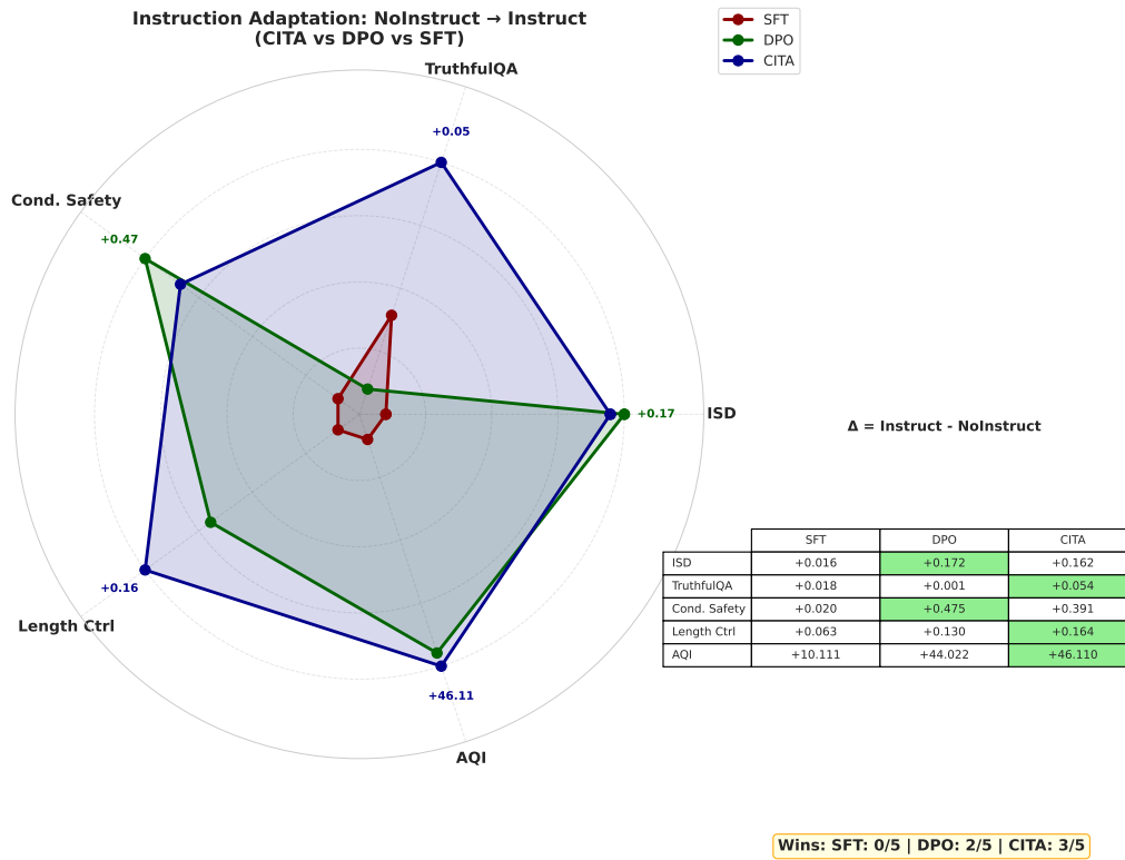
Figure 9: Instruction Adaptation Radar: CITA wins 3/5 benchmarks, DPO wins 2/5, SFT wins 0/5. Values show NoInstruct → Instruct improvement.
