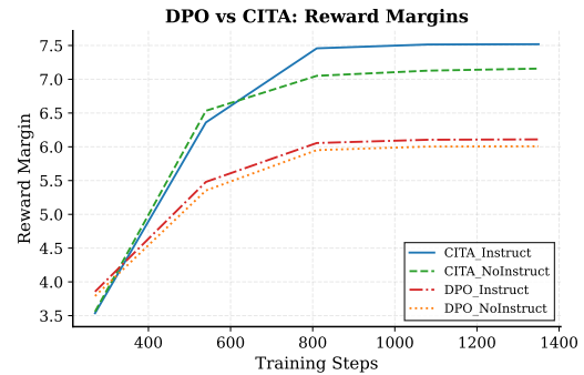
Figure 3: Reward Margins: CITA_Instruct (7.5) > CITA_NoInstruct (7.1) > DPO (~6.0). Higher margins indicate stronger preference learning.
