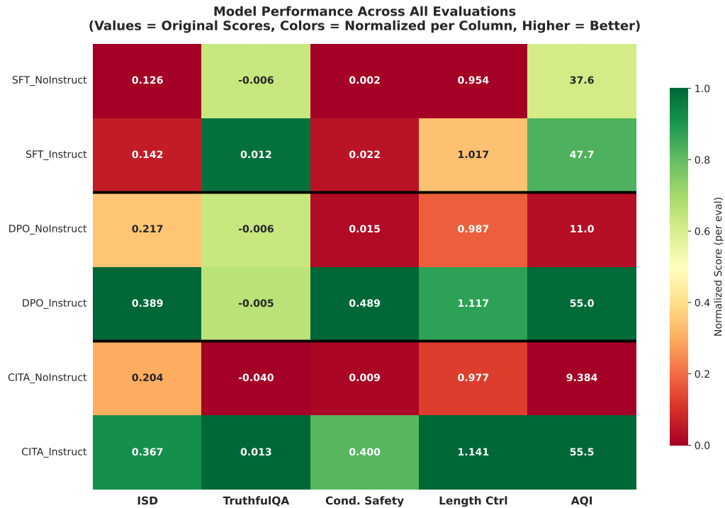
Figure 10: Performance Heatmap: Original scores with column-normalized colors. Green = best, red = worst per benchmark.
