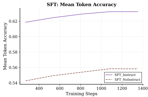
Figure 18: SFT Token Accuracy: SFT_Instruct (63%) achieves higher mean token accuracy than SFT_NoInstruct (56%). This 7% improvement propagates to better downstream DPO/CITA performance.
