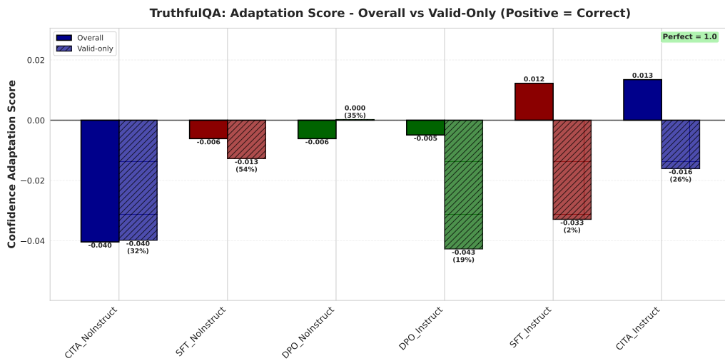
Figure 5: TruthfulQA: Only CITA_Instruct (+0.013) and SFT_Instruct (+0.012) achieve positive adaptation scores (correct uncertainty direction). DPO fails to adapt.
