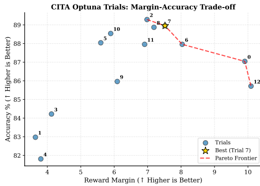
Figure 12: Pareto Frontier: Margin vs. accuracy trade-off across trials. Trial 7 lies on the Pareto frontier, achieving near-optimal balance (margin=7.52, accuracy=89%).
