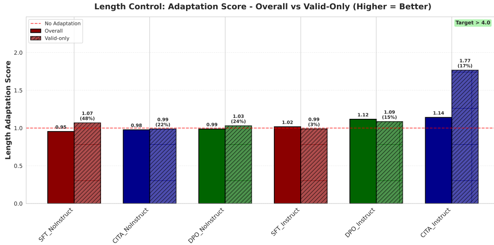
Figure 7: Length Control: CITA_Instruct valid-only (1.77) shows strongest adaptation. Red dashed line = no adaptation baseline (ratio = 1.0).
