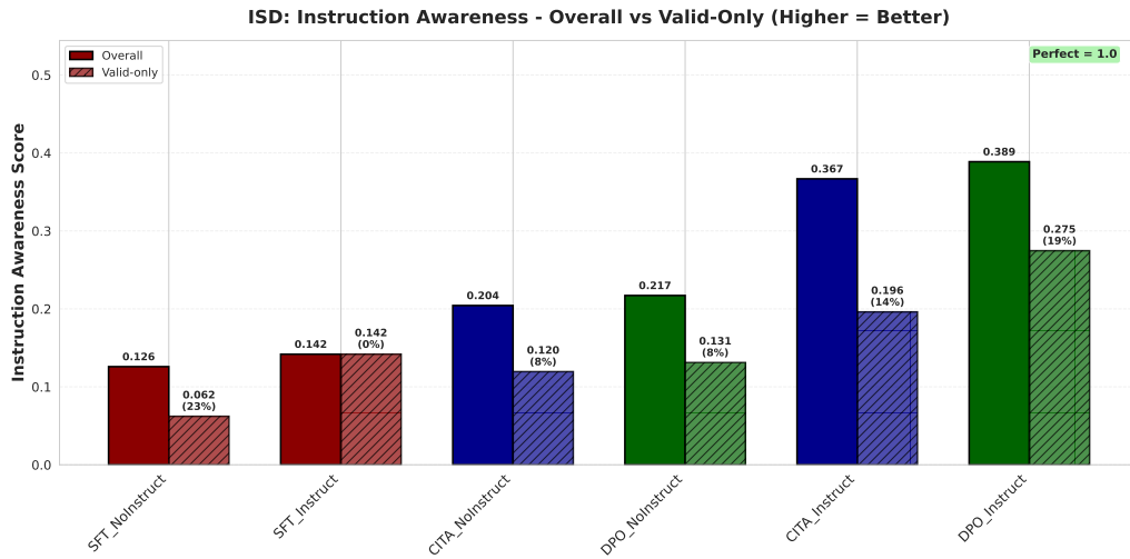
Figure 4: ISD Results: DPO_Instruct (0.389) and CITA_Instruct (0.367) show highest instruction awareness. Hatched bars show valid-only scores with response validity rates.
