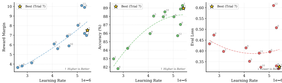
Figure 20: Learning Rate Sensitivity: Reward margin highly sensitive to LR—optimal \sim 5 \times 10^{-6} . Accuracy drops at higher LRs. Key insight: CITA_Instruct requires \sim 50\% lower LR than standard DPO due to 30–40% longer instruction-augmented sequences.
