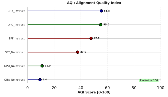
Figure 13: AQI Lollipop : Alignment quality scores emphasizing CITA and DPO performance gap.
