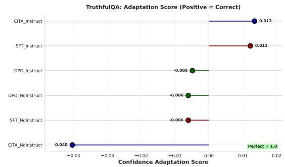
Figure 7: TruthfulQA Lollipop: Adaptation scores highlighting CITA's superior uncertainty calibration.
