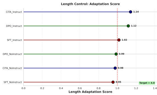
Figure 11: Length Control Lollipop : Response length adaptation ratios with baseline reference.
