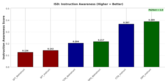
Figure 4: ISD Results: DPO_Instruct (0.389) and CITA_Instruct (0.367) show highest instruction awareness.
