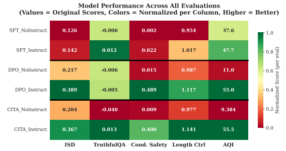
Figure 15: Performance Heatmap : Original scores with column-normalized colors. Green = best, red = worst.
