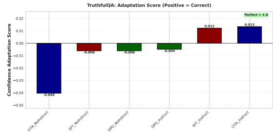
Figure 6: TruthfulQA: Only CITA_Instruct (+0.013) and SFT_Instruct (+0.012) achieve positive adaptation scores.
