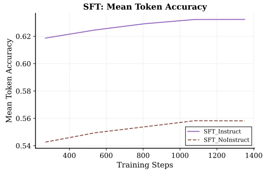
Figure 23: SFT Token Accuracy : SFT_Instruct (63%) achieves higher mean token accuracy than SFT_NoInstruct (56%). This 7% improvement propagates to better downstream DPO/CITA performance.
