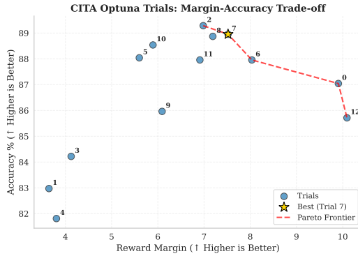
Figure 17: Pareto Frontier: Margin vs. accuracy trade-off across trials. Trial 7 lies on the Pareto frontier, achieving near-optimal balance (margin=7.52, accuracy=89%).
