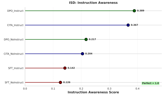
Figure 5: ISD Lollipop: Instruction sensitivity scores with emphasis on relative differences.
