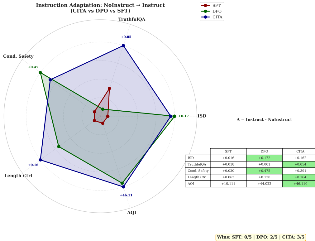
Figure 14: Instruction Adaptation Radar : CITA wins 3/5 benchmarks, DPO wins 2/5, SFT wins 0/5. Values show NoInstruct → Instruct improvement.
