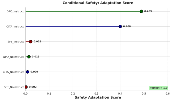
Figure 9: Conditional Safety Lollipop : Safety adaptation scores across STRICT vs. PERMISSIVE contexts.
