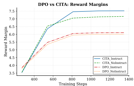
Figure 3: Reward Margins: CITA_Instruct (7.5) > CITA_NoInstruct (7.1) > DPO ( \sim 6.0 ). Higher margins indicate stronger preference learning.
