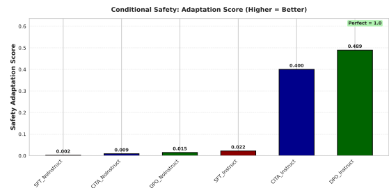
Figure 8: Conditional Safety: DPO_Instruct (0.489) and CITA_Instruct (0.400) show behavioral gap between STRICT vs. PERMISSIVE.
