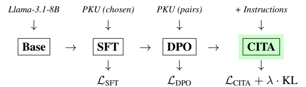
Figure 1: CITA training pipeline. Each stage uses the previous checkpoint. CITA adds mandatory KL regularization for instruction-conditioned alignment.
