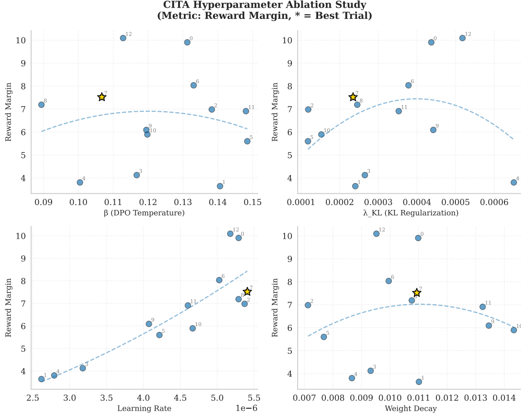
Figure 16: Hyperparameter Ablation Study: Reward margin sensitivity to \beta , \lambda_{KL} , learning rate, and weight decay across 13 Optuna trials. Trial 7 (★) achieves the best trade-off. Key findings: (a) \beta \in [0.10, 0.12] yields highest margins; (b) \lambda_{KL} \approx 0.0002 balances stability and performance; (c) Learning rate sensitivity is high— \sim 5e-6 is optimal for instruction-augmented training; (d) Weight decay shows moderate sensitivity with optimal range \sim 0.01 .
