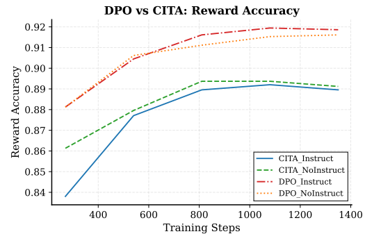
Figure 2: Reward Accuracy: All models converge to 89–92%. DPO variants achieve slightly higher accuracy.
