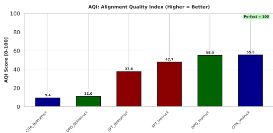
Figure 12: AQI : CITA_Instruct (55.5) and DPO_Instruct (55.0) achieve highest clustering scores.
