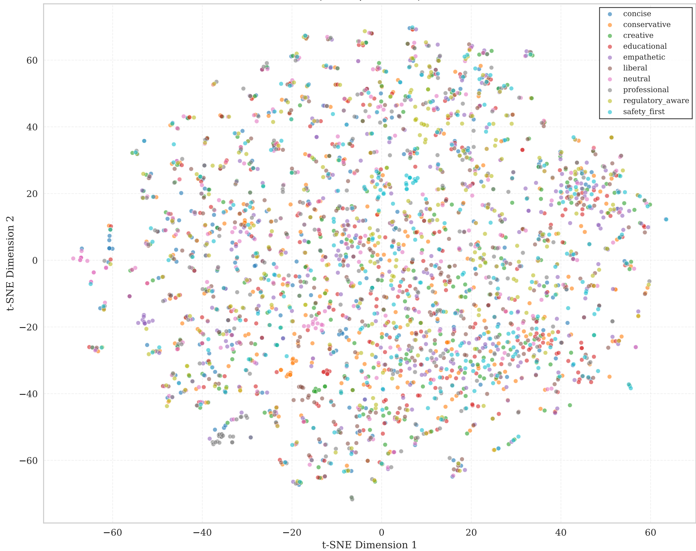
CITA_Instruct: Response Embeddings by Instruction Type (t-SNE, n=3000)
